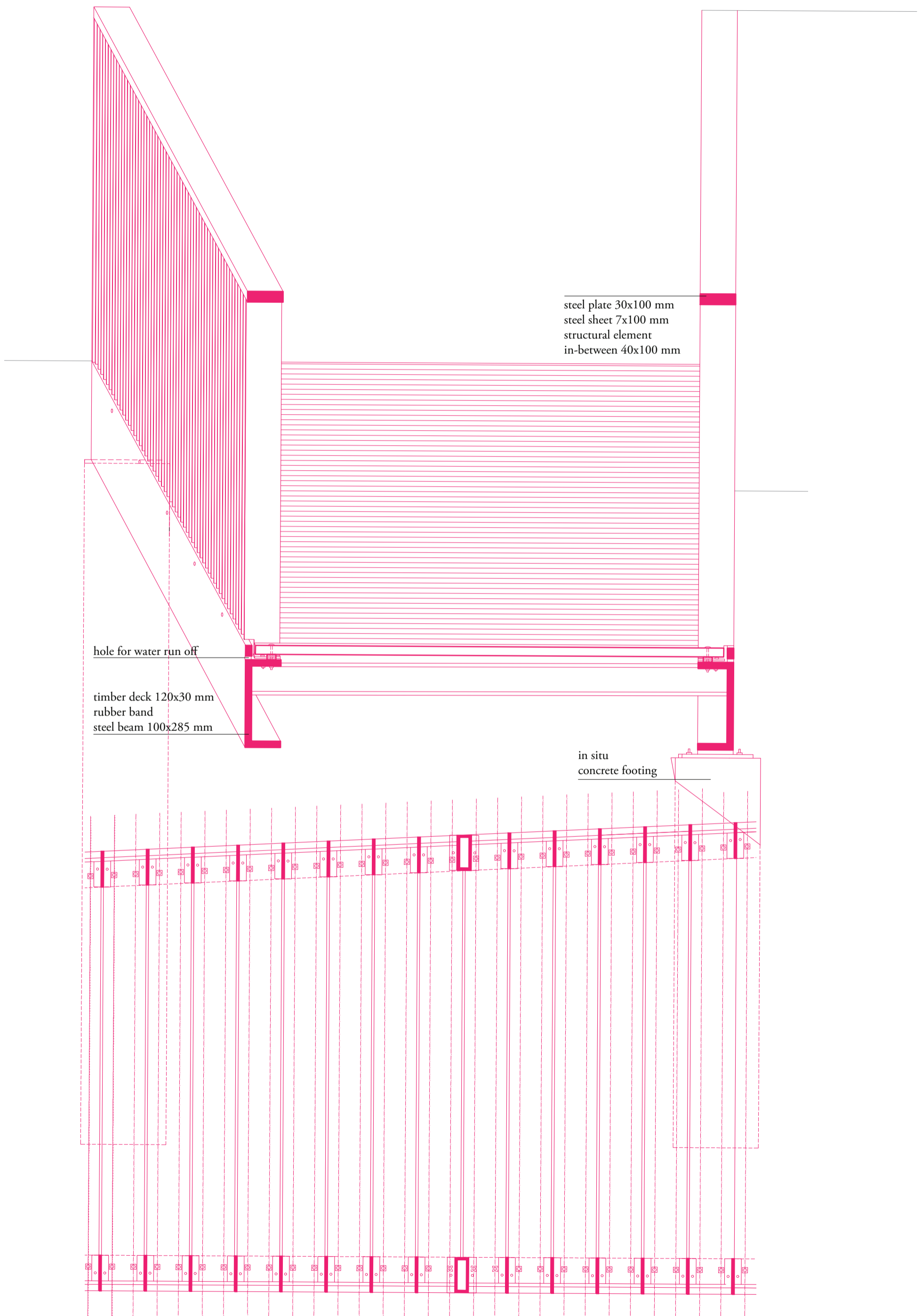
Path section and elevation 1:10
