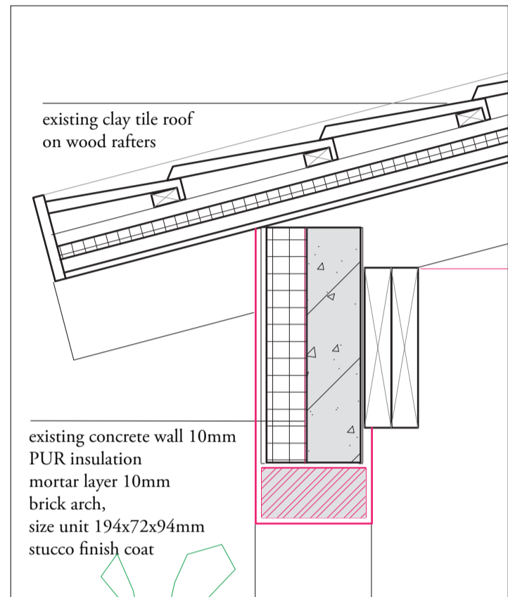
Detail 1 1:10
