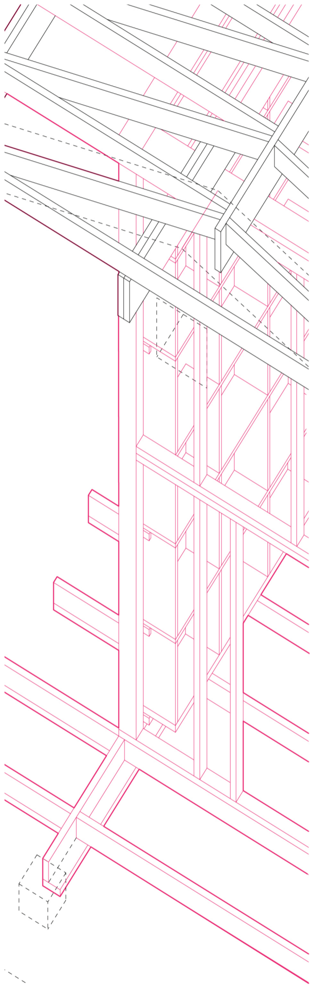
Old and new timber structures in the box-in-a-box construction
