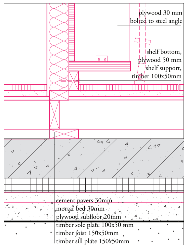
Detail 2 1:10
