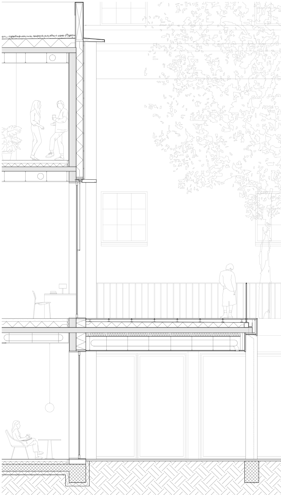
facade fragment
