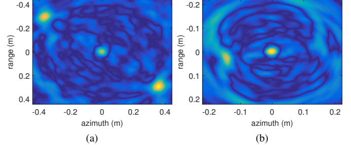
Fig. 15. Inverse Radon image with different ambiguity number. (a) The ambiguity number is 2; (b) The ambiguity number is 1.
