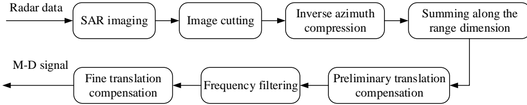
Fig. 11. Flowchart of m-D signal extraction for SAR data.
