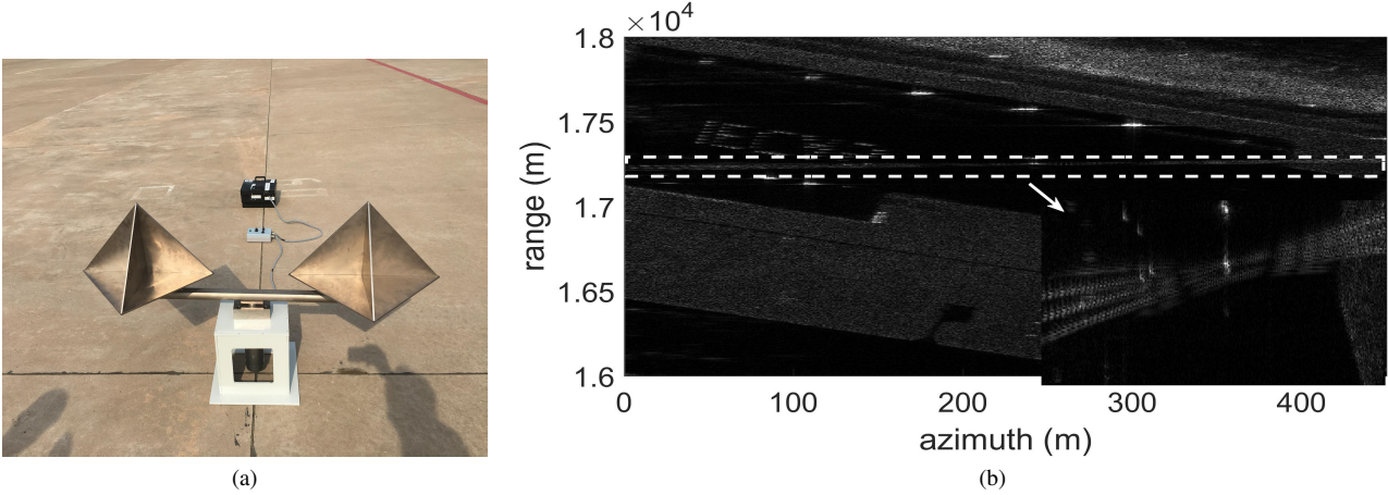
Fig. 10. The rotating corner reflectors located in the airport. (a) the rotating corner reflectors; (b) SAR image of the interesting area.
