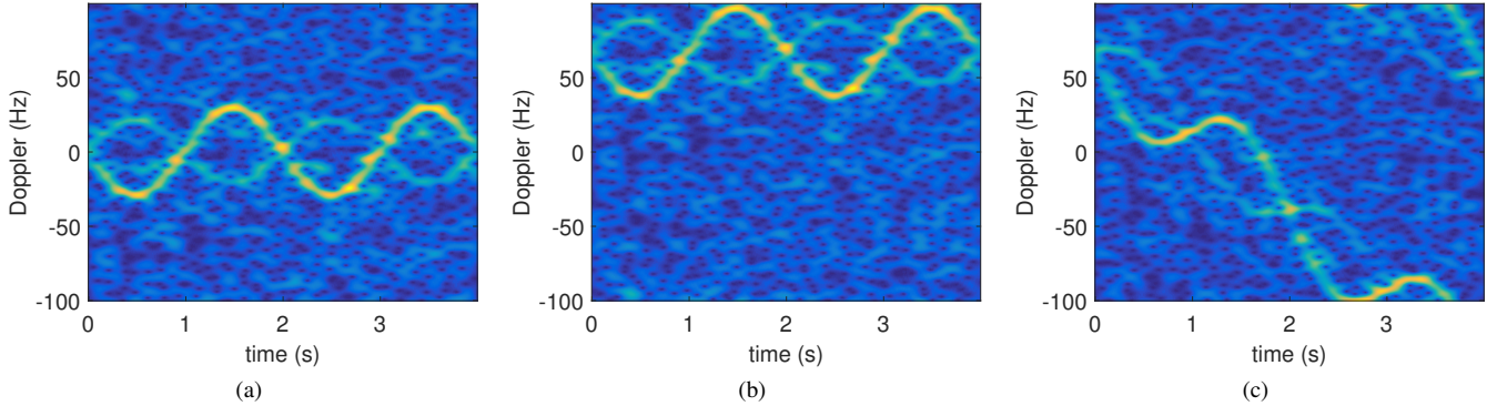
Fig. 4. STFT of the radar echo.(a) the MM case; (b) the MMLT case; (c) the MMQT case.
