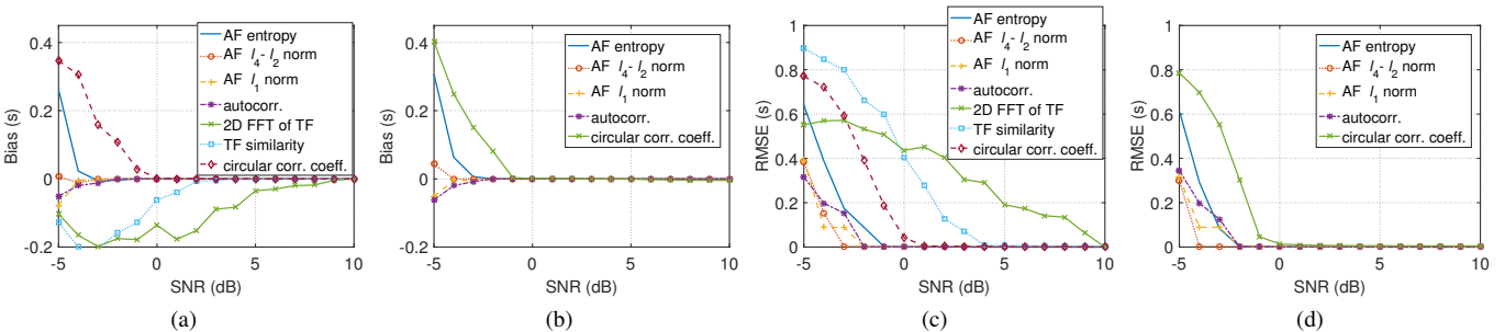
Fig. 7. Bias and RMSE versus SNR. (a) Bias for the MMLT case; (b) Bias for the MMQT case; (c) RMSE for the MMLT case; (d) RMSE for the MMQT case.
