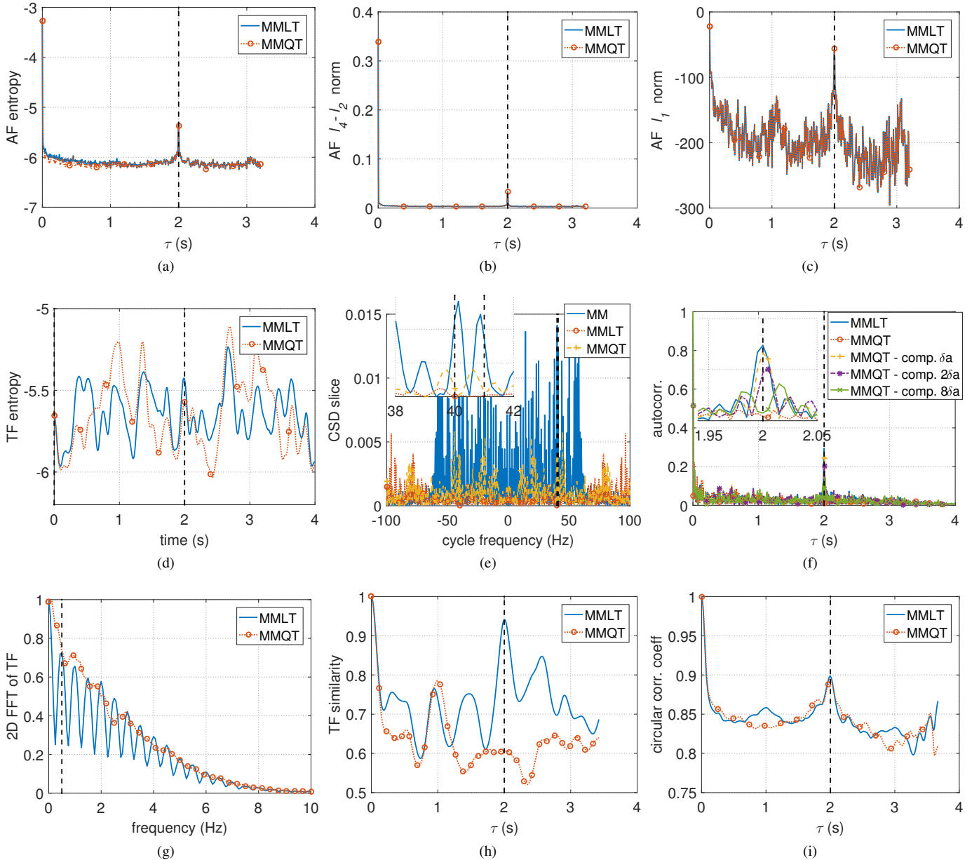
Fig. 6. Estimation Statistics. (a) AF entropy; (b) AF l_4-l_2 norm; (c) AF l_1 norm; (d) TF entropy; (e) slices of CSD; (f) autocorrelation (the dash-dot lines with circle, square and asterisk markers denote the results by integrating translation compensation with different search intervals); (g) 2D FFT of TF; (h) TF similarity; (i) circular correlation coefficients. The true m-D period/frequency is indicated by a black dashed vertical line in (a), (b), (c), (f), (g), (h), (i). While in (d) and (e), two vertical lines with distance of the true m-D period and two multiples of the m-D frequency are plotted which means that the statistics should have periodic peaks or periodic pattern at these two instants if they are effective.
