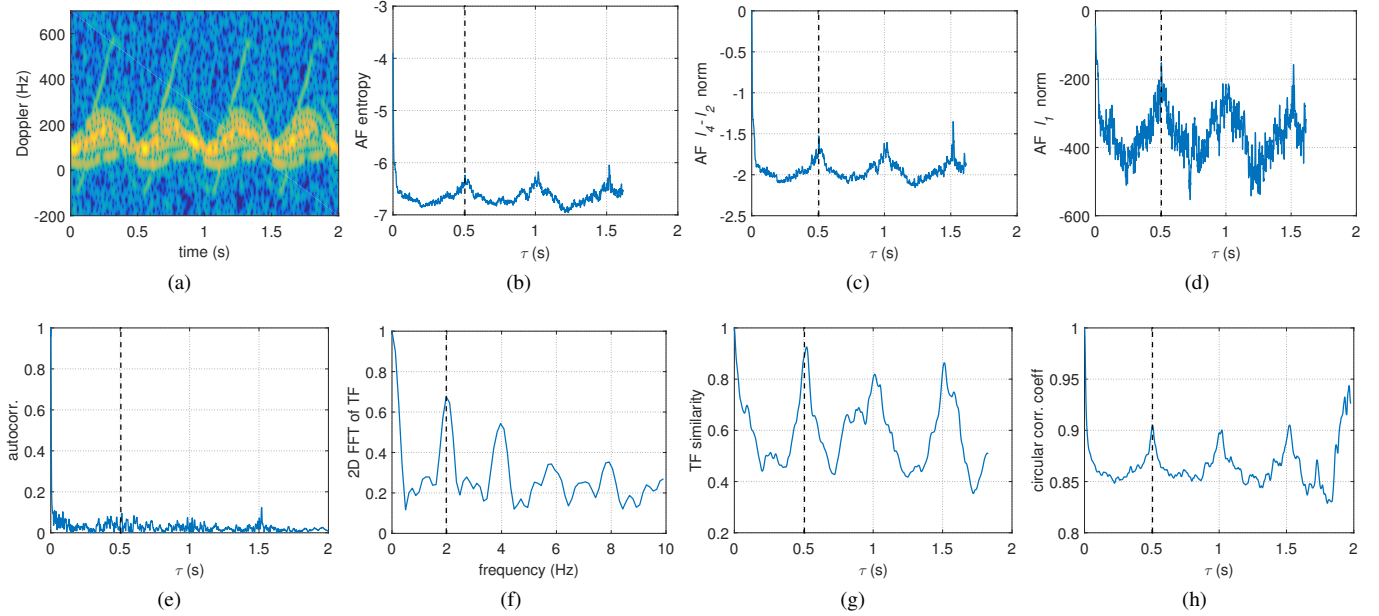
Fig. 9. Period estimation results of the walking human. (a) TF of the m-D signal; (b) AF entropy; (c) AF l_4-l_2 norm; (d) AF l_1 norm; (e) autocorrelation; (f) 2D FFT of TF; (g) TF similarity; (h) circular correlation coefficients. The black dashed vertical line in the figure has the same meaning with that of Fig. 6.
