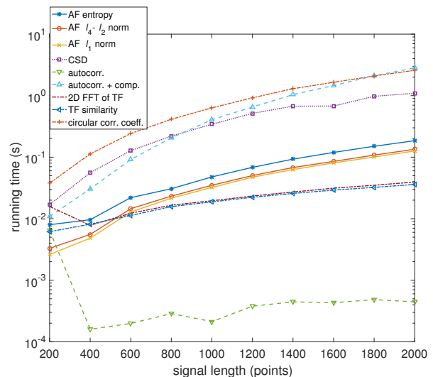
Fig. 8. Running time of the estimation methods.
