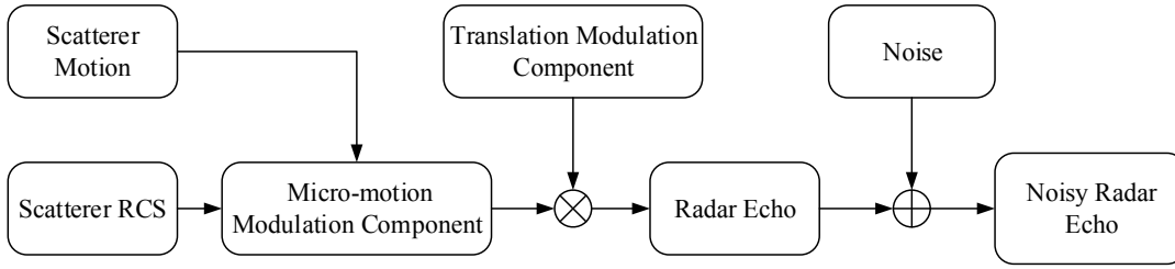
Fig. 3. Flowchart of the coning motion simulation.
