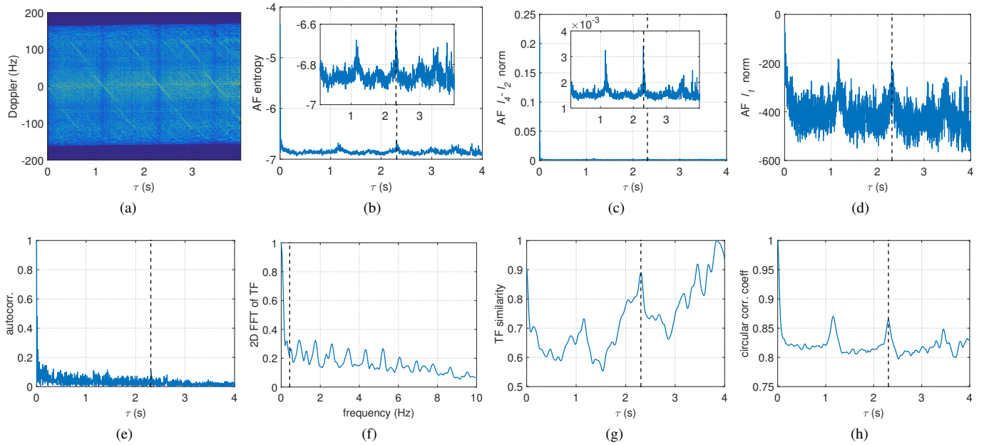
Fig. 13. (a) AF of the m-D signal; (b) AF entropy; (c) AF l_4-l_2 norm; (d) AF l_1 norm; (e) autocorrelation; (f) 2D FFT of TF; (g) TF similarity; (h) circular correlation coefficients. The black dashed vertical line in the figure has the same meaning with that of Fig. 6.
