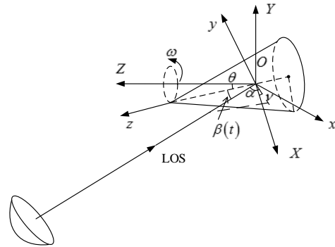
Fig. 2. The cone target model.
