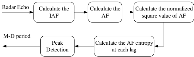
Fig. 1. Flowchart of AF entropy-based m-D period estimation.
