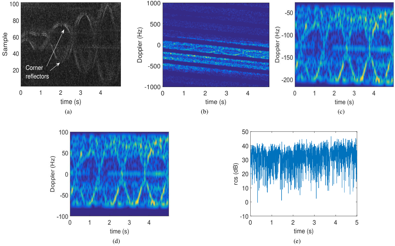
Fig. 12. (a) range-compressed and azimuth-uncompressed signal; (b) STFT of the azimuth signal; (c) STFT of the preliminary compensated and filtered azimuth signal; (d) STFT of the m-D signal; (e) the uncalibrated RCS of the target.
