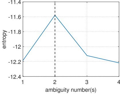
Fig. 14. The entropy of the inverse Radon image. The true ambiguity number is indicated by the black dash vertical line.
