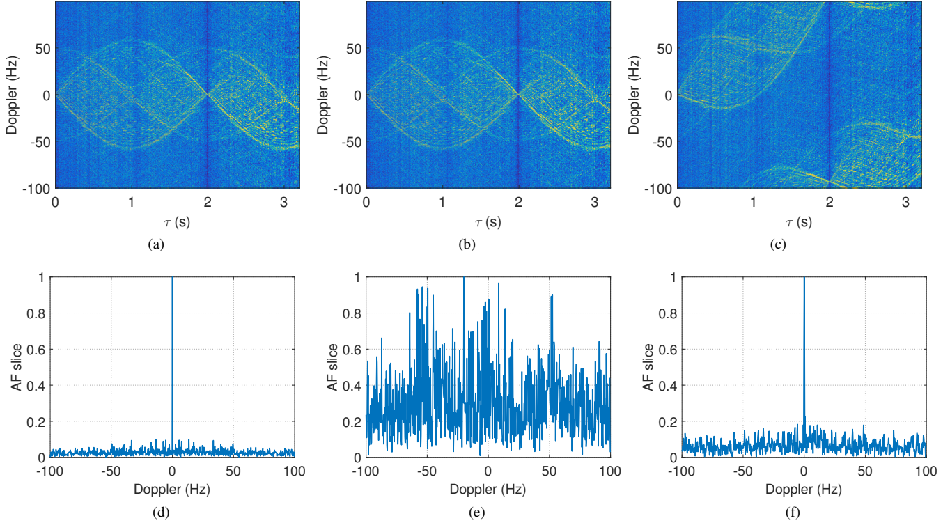
Fig. 5. AF of the radar echo. (a) the MM case; (b) the MMLT case; (c) the MMQT case; (d) slice of the MM case at \tau = 0 s; (e) slice of the MM case at \tau = 1 s; (f) slice of the MM case at \tau = 2 s.
