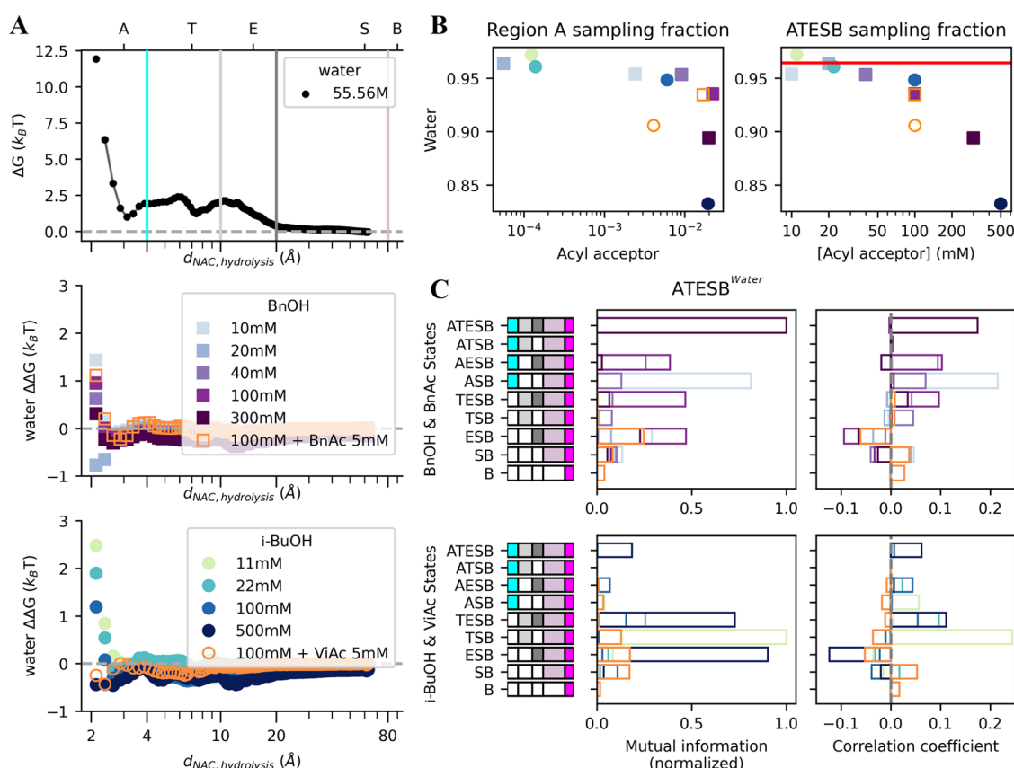
Figure 4. Binding mechanism of water. (A) Binding free energy profiles of d_{NAC} for pure water (top) and under the presence of BnOH (middle) and i -BuOH (bottom). Circles correspond to the mean \Delta G values (in k_B T units) per d_{NAC} shell over all calculated protein–substrate pairs, subunits, and replicates. Shaded regions correspond to the associated standard deviations. A, T, E, and S d_{NAC} shell maximal radii in solid lines: A—cyan, T—light gray, E—dark gray, S—gray, and B—pink. Values of d_{NAC} are represented in the logarithmic scale for clarity. (B) Sampled region A by water as a function of acyl acceptor sampling (left) and sampled ATESB by water as a function of acyl acceptor concentration (right). (C) Mutual information (left) and correlation coefficients (right) between water ATESB states and BnOH, i -BuOH states.
