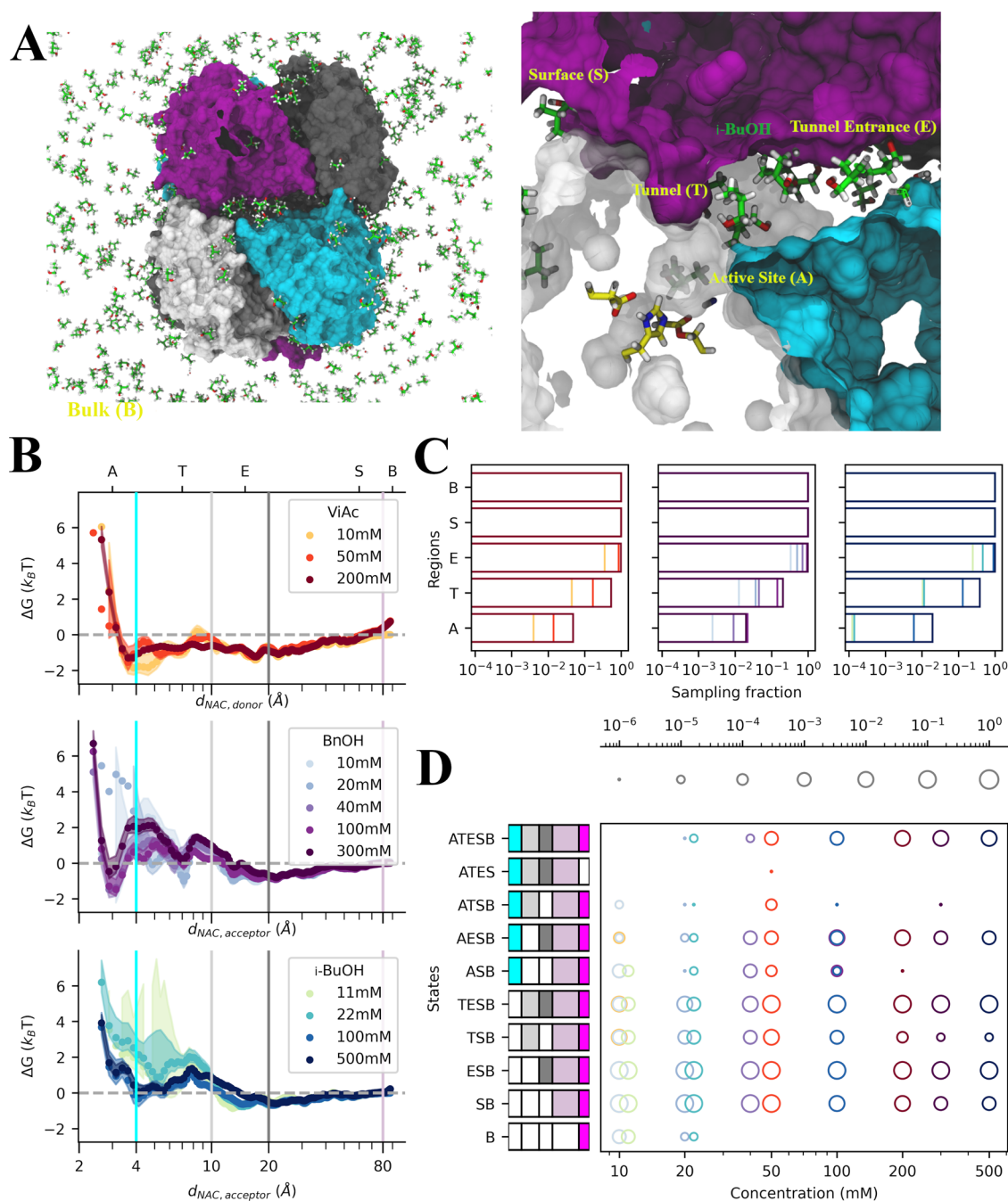
Figure 3. Binding mechanism of transesterification substrates. (A) Snapshot of substrate i -BuOH distribution in the MsAcT surface and within the active site tunnel. i -BuOH molecules are shown in green licorice representation. Corresponding locations along d_{NAC} regions have yellow labels. (B) Binding free energy profiles of d_{NAC} as a function of substrate concentration. Circles correspond to the mean \Delta G values (in k_B T units) per d_{NAC} shell over all calculated protein–substrate pairs, subunits, and replicates. Shaded regions correspond to the associated standard deviations. A, T, E, and S d_{NAC} shell maximal radii in colored solid lines: A—cyan, T—light gray, E—dark gray, S—gray, and B—pink. Values of d_{NAC} are represented in the logarithmic scale for clarity. (C) Sampled regions as a function of substrate concentration. (D) Sampled states as a function of concentration. Circles correspond to the sampling fraction in logarithmic scale for clarity.
