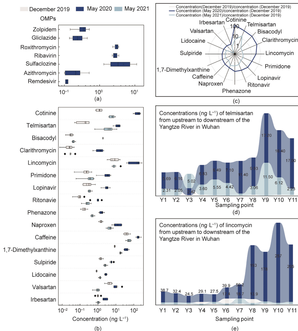
Fig. 2. (a) 7 OMPs detected in the Yangtze River in May 2020. (b) 16 OMPs showed significantly higher concentrations in the Yangtze River in May 2020 than in December 2019 and May 2021. (c) Ratio of the OMP concentration in December 2019, May 2020, and May 2021 to the OMP concentration in December 2019. Concentrations of (d) telmisartan and (e) lincomycin from upstream to downstream of the Yangtze River in December 2019, May 2020, and May 2021.
