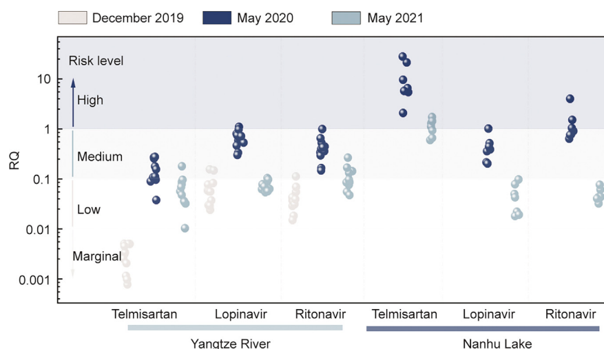
Fig. 4. Changes in the ecological risk of the OMPs in the Yangtze River and Nanhu Lake in Wuhan based on the comparison of RQ values.
