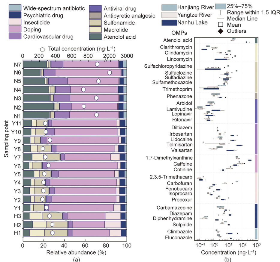
Fig. 1. (a) Compositional profiles and (b) concentrations of 33 OMPs in the Hanjiang River, Yangtze River, and Nanhu Lake in Wuhan in May 2021. IQR: interquartile range.
