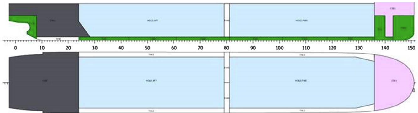
Fig. 2. Layout of ship 2, including a side view and a top view. The scale along the length of the ship represents the frames, with a spacing distance of 0.7 m between frames 24 and 104 and 0.6 m for the remaining frames. The blue areas are the cargo holds. The grey area is the engine room. The pink area is service space. The white areas are void space. The green areas are ballast tanks. This figure has been provided by DEKC Maritime.
