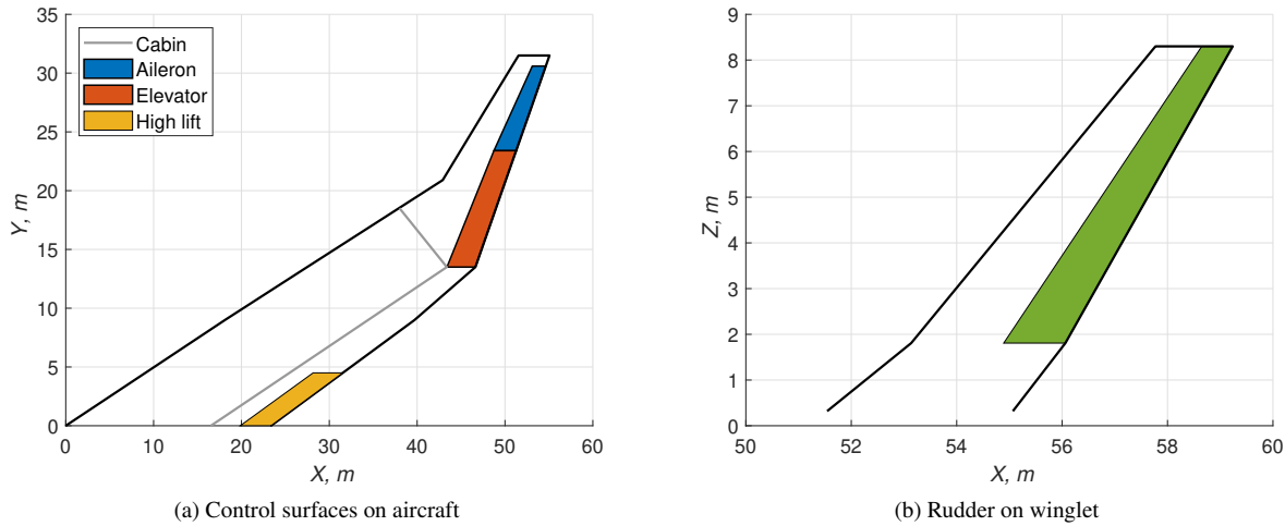
Fig. 8 Control surfaces identified in this study positioned on the aircraft
