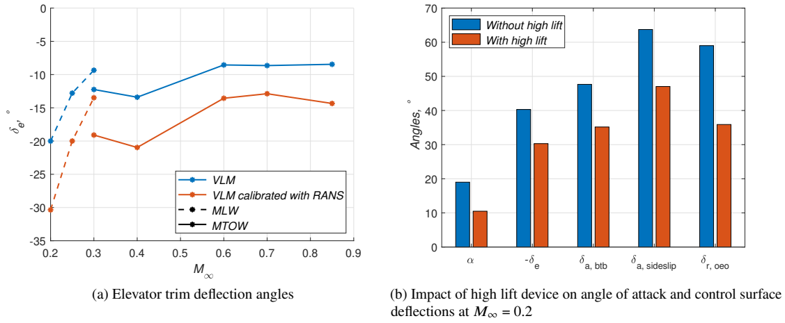
Fig. 7 Elevator deflections for longitudinal trim and impact of high lift device on other control surface requirements
