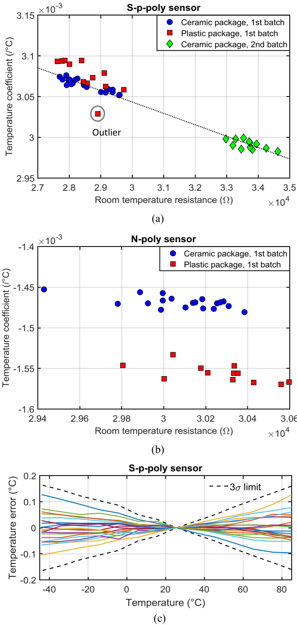
Fig. 16. Correlation between R_0 and its TC for (a) s-p-poly resistor and (b) n-poly resistor. (c) Inaccuracy of s-p-poly sensor after a correlation-assisted one-point calibration (ceramic packaged, first batch).
