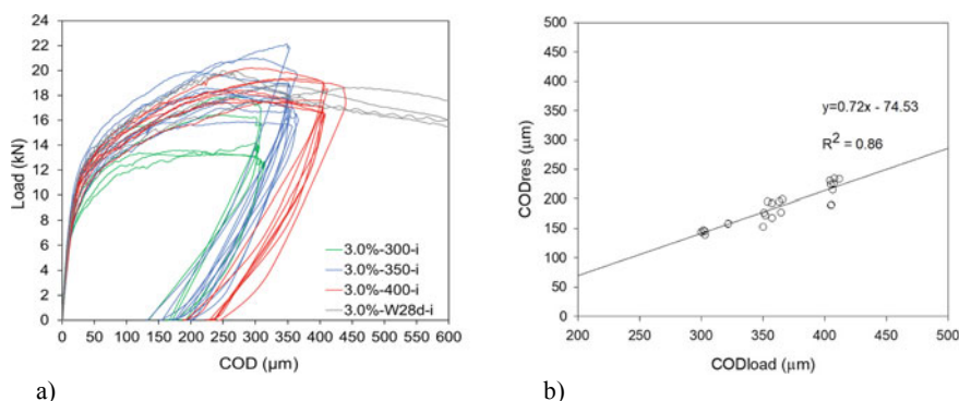
Fig. 4 a Load-displacement curves obtained at 28 days while establishing target COD_{load} of 300, 350 and 400 μm; and b relation between COD_{load} and COD_{res}
