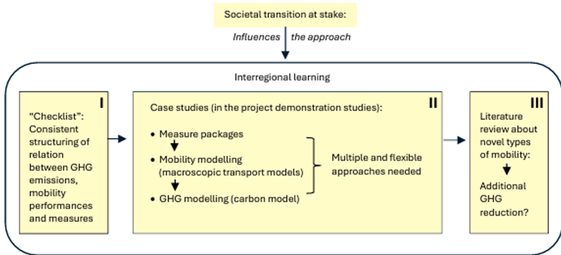
Fig. 1. Research approach.
