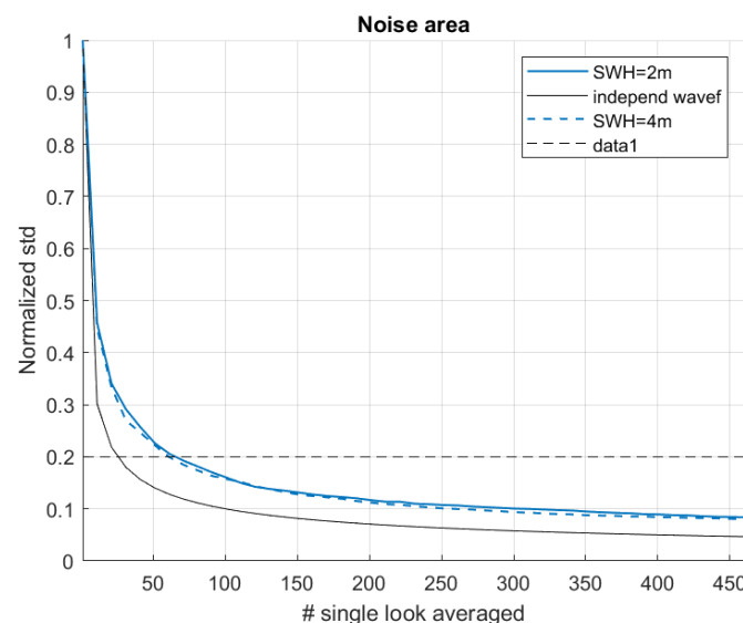
Figure 8. Normalized standard deviation evolution with regards to the level of multilooking of FF single-looks. Three scenarios are plotted: theoretical decrease with independent single-looks (in black solid line), FF oceanic real data with SWH around 2m (blue solid line) and FF oceanic real data with SWH around 4m (in blue dashed line). We aim to measure the posting rate corresponding to a noise reduction of 80% represented by the horizontal black dashed line.
