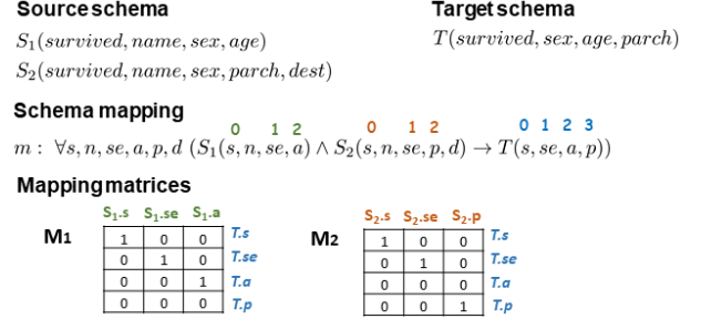
Figure 1: Schema mapping and mapping matrices
