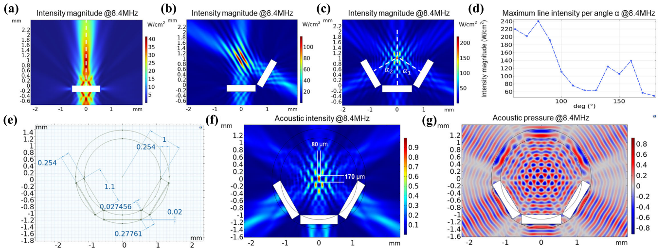
Fig. 2. Simulation results (a)–(c) show the focal spot size and acoustic intensity for one, two, and three PZT-based US transducers in a curved configuration. (d) Relation between the angle between three PZT-based US transducers and the maximum acoustic intensity magnitude. (e) Dimensions for the simulated cuff design, whereas (f) and (g) show the acoustic intensity magnitude and pressure profiles, respectively.
