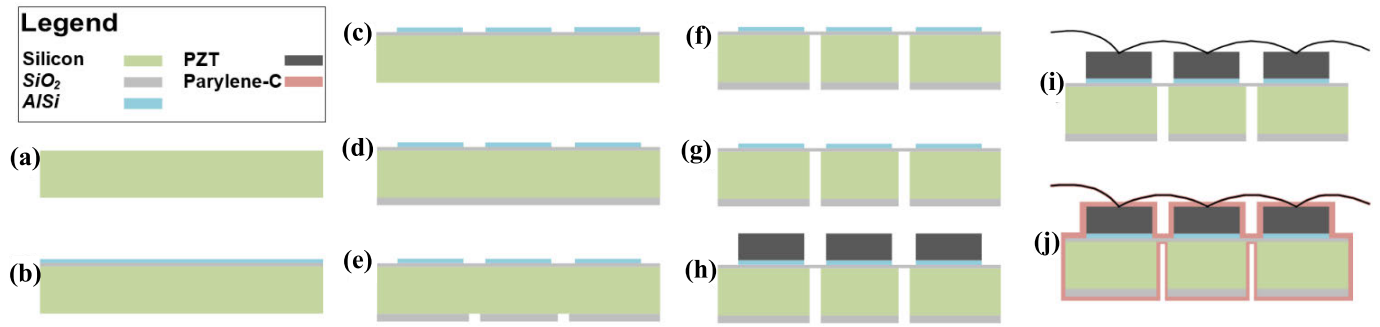
Fig. 4. Wafer-level microfabrication process steps. (a) Process starts with a wafer on which alignment markers are etched. (b) Layer of SiO 2 and on top a layer of AlSi is deposited. (c) AlSi layer is patterned. (d) SiO 2 layer is deposited at the backside. (e) SiO 2 at the backside is patterned. (f) Silicon substrate is etched from the backside. (g) Wafer is diced. (h) PZTs are placed on top. (i) Tungsten wire is attached on top of the PZTs. (j) Device is encapsulated with parylene-C.
