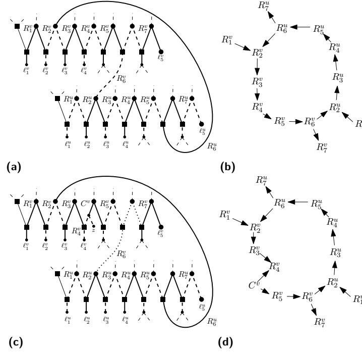
■ Figure 5 Cherry cover of \text{Gad}(v) and \text{Gad}(u) . In (a), the unique cherry cover of the principal part of \text{Gad}(v) and \text{Gad}(u) is displayed, in (b), the cherry cover auxiliary graph of (a) is given. In (c), the leaf z \notin X is added to the principal part of \text{Gad}(v) , and one possible cherry cover of the same part of the network is given. And in (d), the cherry cover auxiliary graph of (c) is given.
