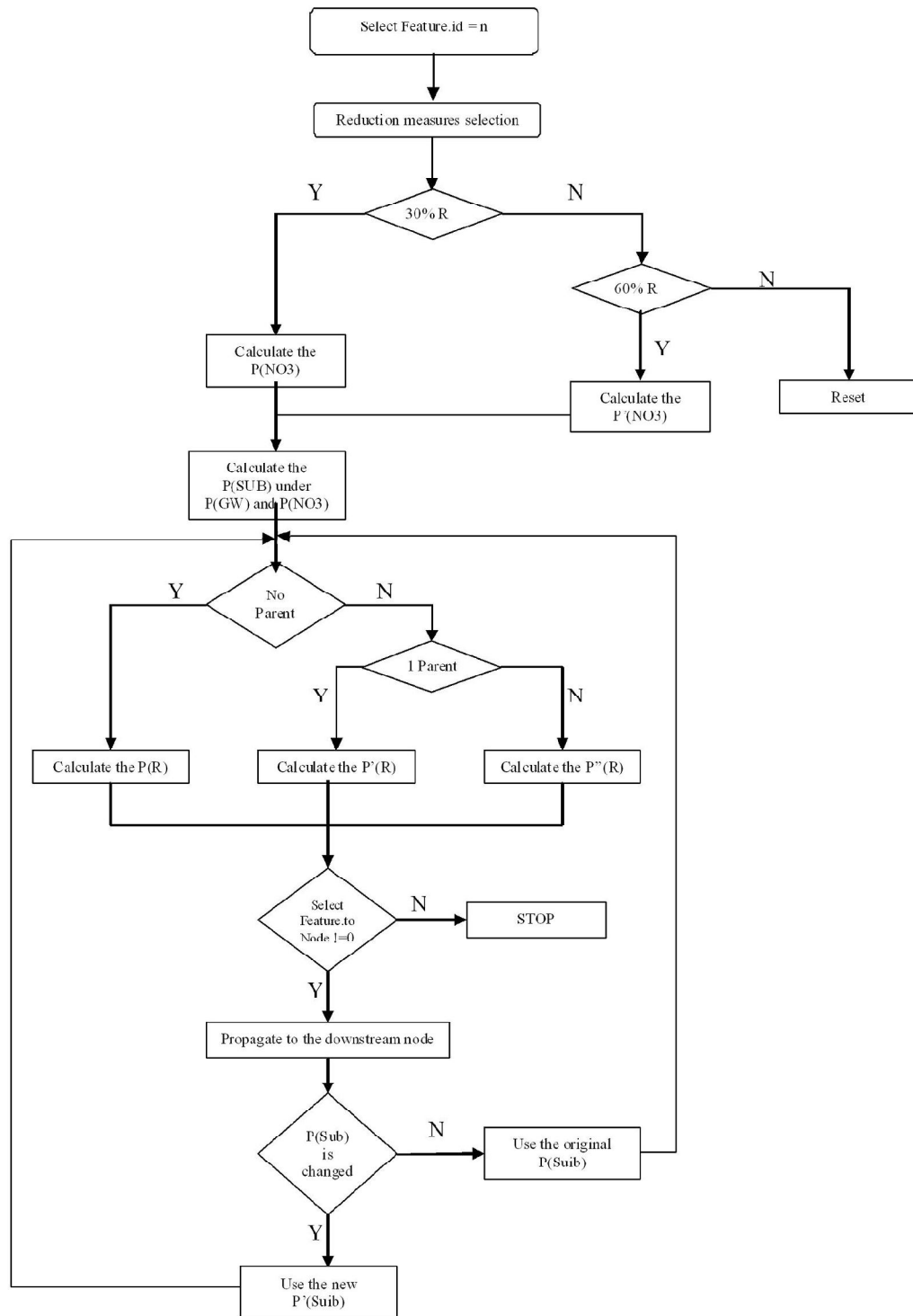
Fig 3.15 Flow Chart of BBN simulation core
