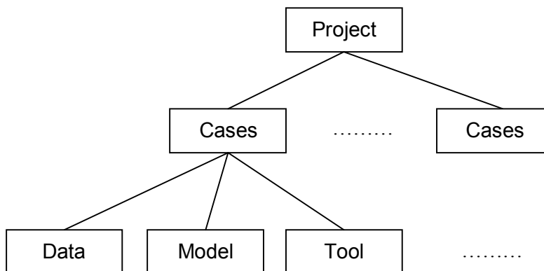
Fig 6.8 Project Structure
