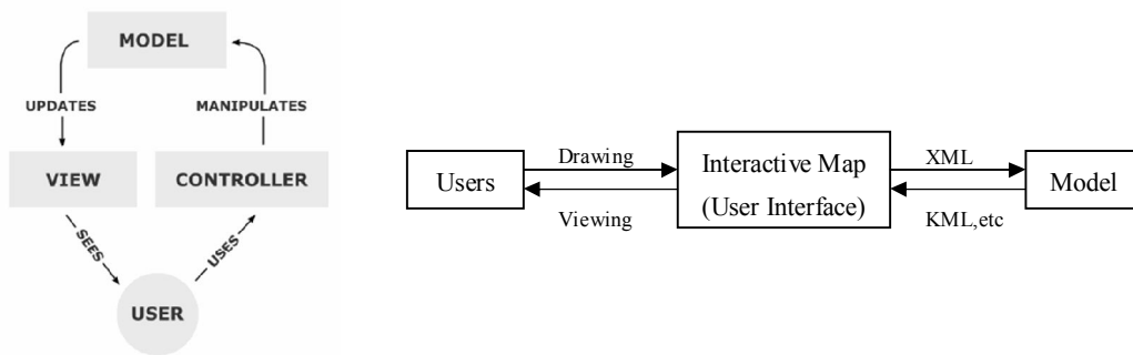
Fig 6.5 MVC pattern
