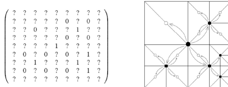
Fig 4.16 A sample triangulation of a 9*9 height field.
