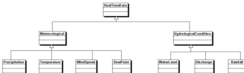
Fig 5.5 Detail Data Model of RealTimeData Module
