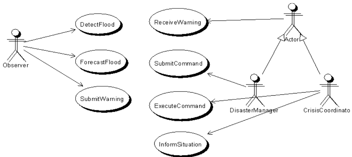
Fig 5.3 Use Case Diagram for the concept design
