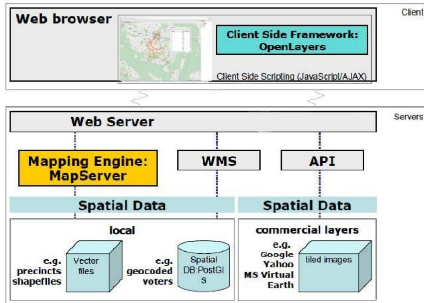
Fig 3.6 Stucuture of VisREACHER
