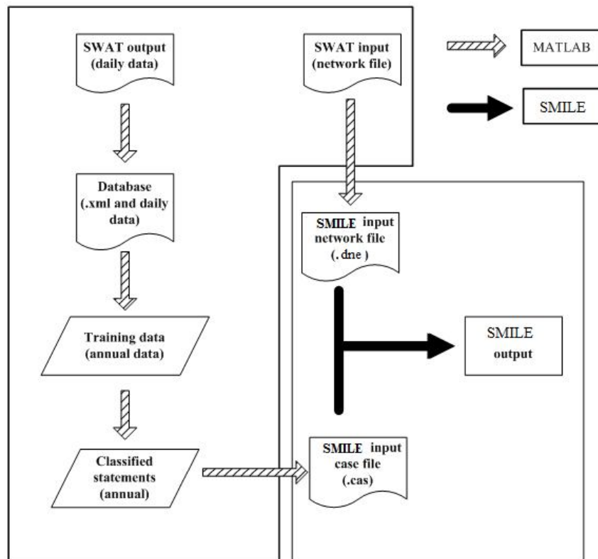
Fig 3.3 Process Flowchart of REACHER
