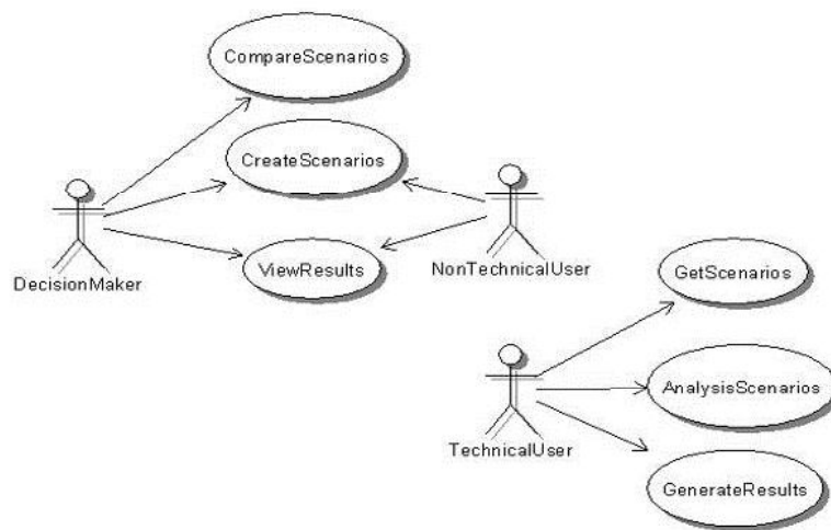
Fig 6.4 Use Case model for different users
