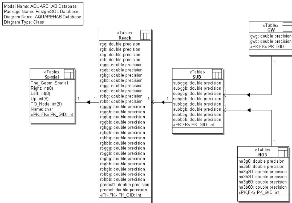
Fig 3.13 Sturcture of the Database
