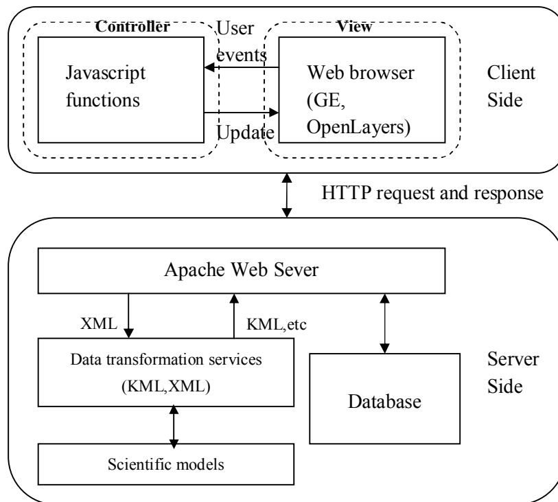
Fig 6.6 Overall architecture of the prototype
