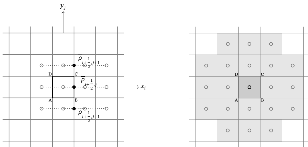
Figure 3.2: Left Grid points at cell-centers required to compute \langle \partial p / \partial x \rangle_{i+1/2,j} using (3.18). Right A 5 \times 5 block required to compute the flux divergence of cell ABCD.
