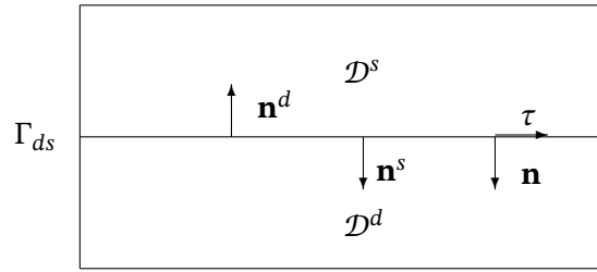
Figure 5.1: Geometry of the Darcy-Stokes problem coupled with the transport equation. Subdivision of the domain \mathcal{D} into a free-flow subregion \mathcal{D}^s and a porous medium subdomain \mathcal{D}^d , by an internal interface \Gamma_{ds} .
