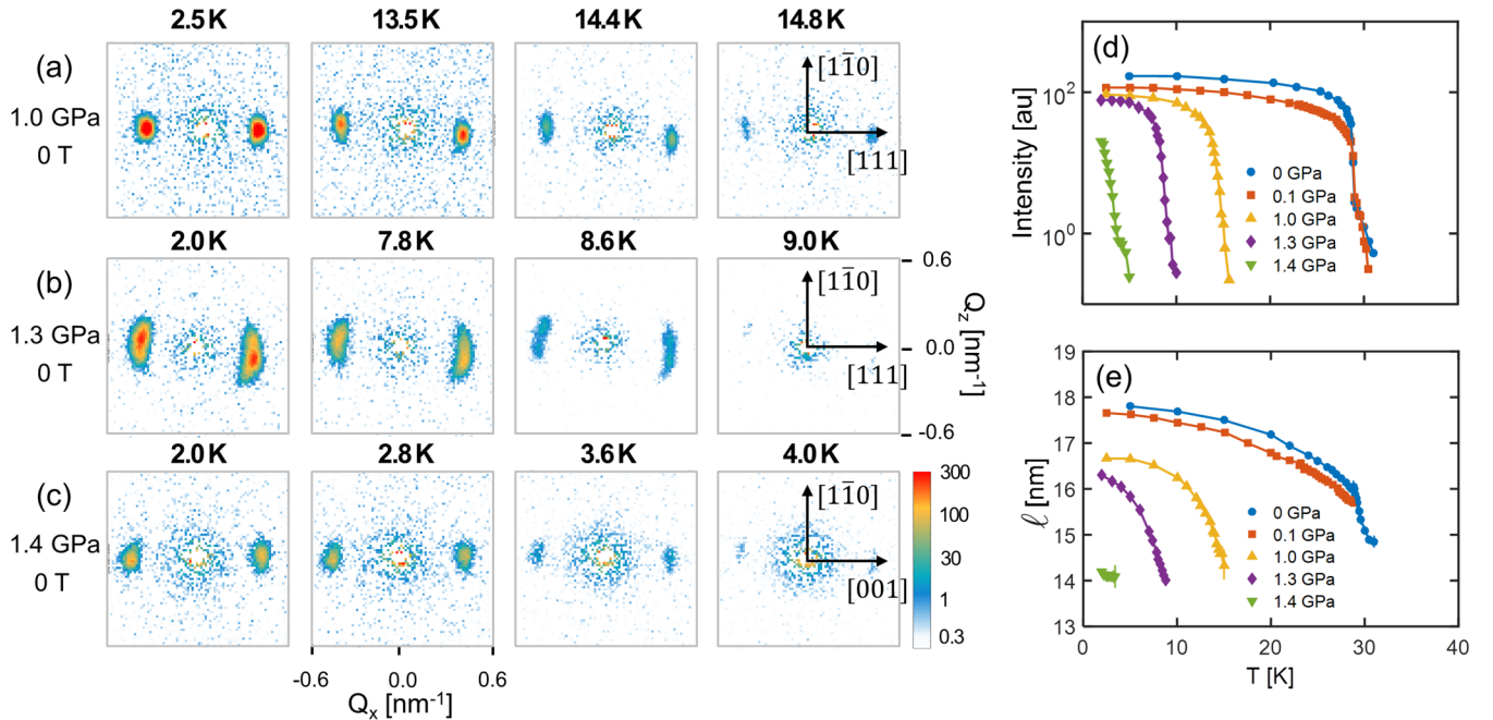
FIG. 2. SANS results at zero magnetic field. (a)–(c) display characteristic SANS patterns obtained at a pressure of (a) p = 1.0 GPa, (b) 1.3 GPa, and (c) 1.4 GPa and for the temperatures indicated. (d) displays the total scattered intensity as a function of temperature for the pressures indicated in the figure legend. The total scattered intensity is obtained by summing all the intensity of the SANS patterns. (e) shows the temperature dependence of the pitch of the helix \ell for the pressures indicated in the figure legend. \ell is obtained from the maximum of a fit of a Gaussian to the radial averaged SANS patterns.
