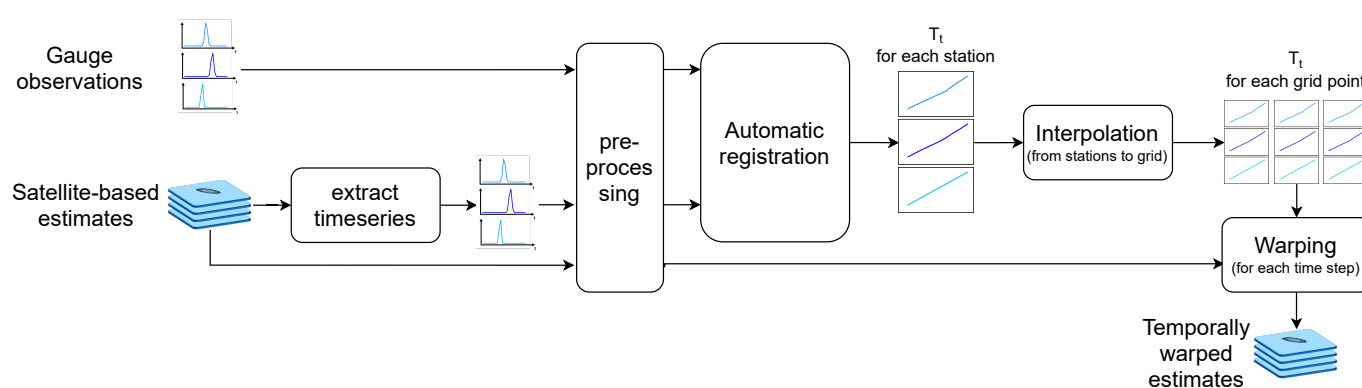
Figure 2. Flowchart of the time warping method.
