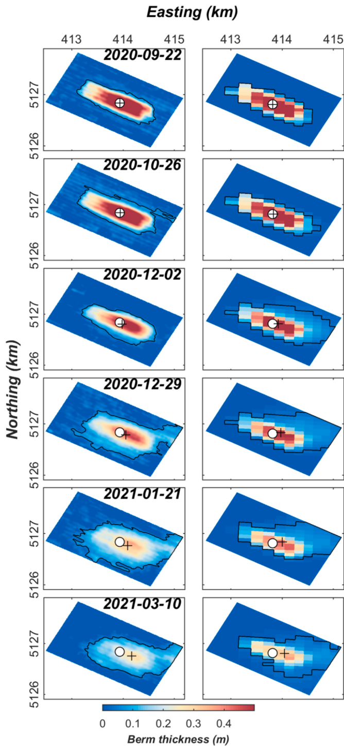
Fig. 7. Observed (left panels) and modeled (right panels) berm morphology over time. Model results derived from simulation with best overall performance (R5, Table 3). Additional caption details as in Fig. 4.
