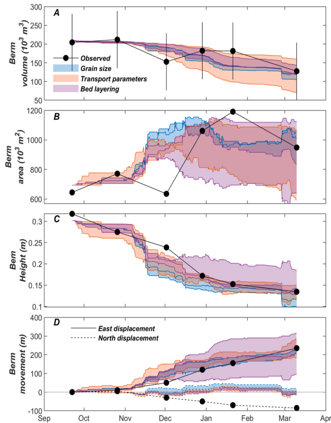
Fig. 6. Comparisons between measured (black dots) and simulated berm morphology metrics (colored lines) including A, berm volume, B, berm area, C, mean berm height, and D, movement of the berm centroid over time. For each morphology metric, model results are shown for simulations with a variety of grain sizes, transport formula coefficients, and bed layer thicknesses. See Table 2 for the parameters used in the model simulations. Error bars in A represent potential bias between initial and successive surveys of \pm 3 cm.
