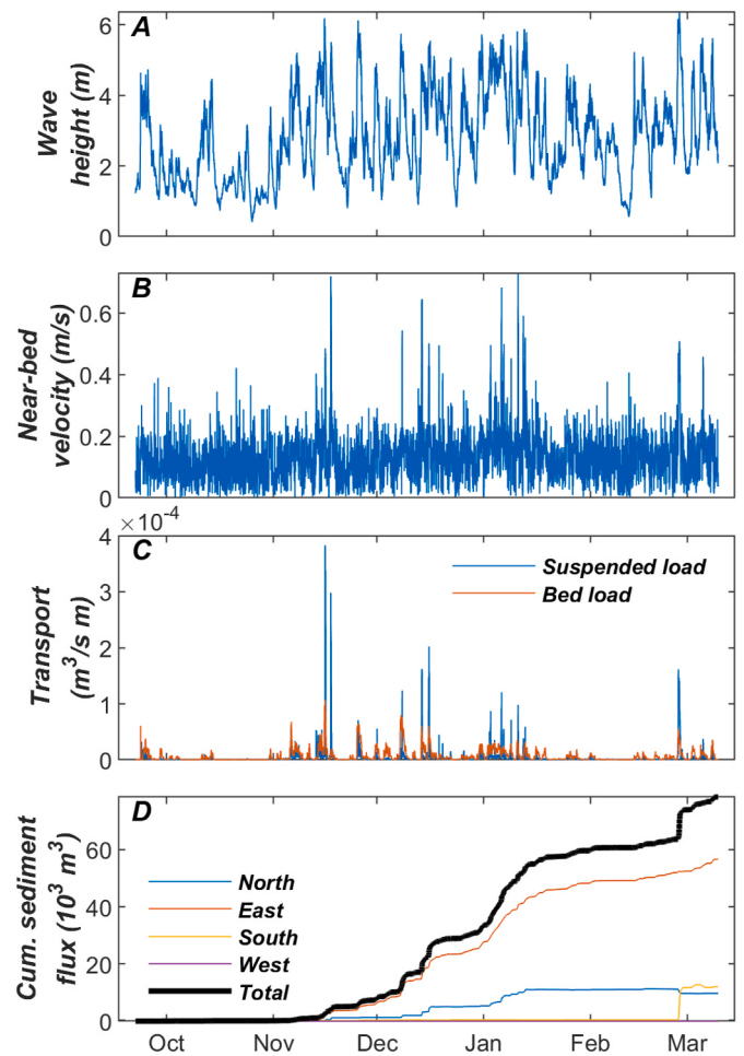
Fig. 8. Time series of, A, significant wave height, B, near-bed current velocity magnitude, C, instantaneous bed- and suspended load transports, and D, cumulative sediment flux through cross sections. Positive cumulative sediment fluxes represent transport out of the initial placement zone. The locations of the cross sections (red lines) and location of time series output (white circle) are provided in Fig. 9A.
