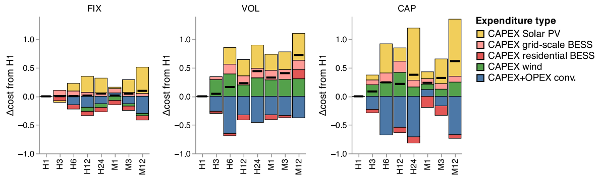
Fig. 9. Normalized change in expenditure of each technology relative to H1 granularity under each tariff, across decreasing temporal granularity of retail electricity prices. Horizontal bars in black illustrate the total increase in cost. FIX: fixed tariff, VOL: volumetric tariff, CAP: capacity tariff, H: hourly temporal granularity, M: monthly temporal granularity.
