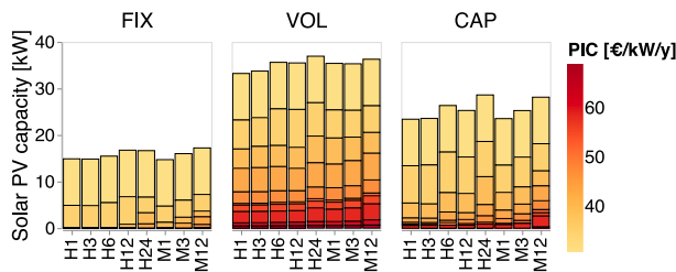
Fig. E.4. Sensitivity analysis results: installed individual consumer solar PV capacities.
