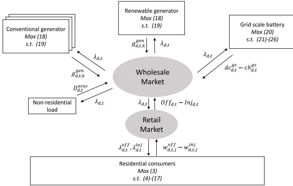
Fig. 1. Schematic overview of the non-cooperative game. Residential consumers will get retail offtake/injection prices while other agents receive wholesale market prices. The offtake/injection prices remain constant per averaging period.
