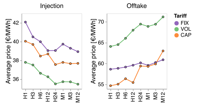
Fig. 5. Average offtake & injection prices under each tariff, across decreasing temporal granularity of retail electricity prices. FIX: fixed tariff, VOL: volumetric tariff, CAP: capacity tariff, H: hourly temporal granularity, M: monthly temporal granularity.
