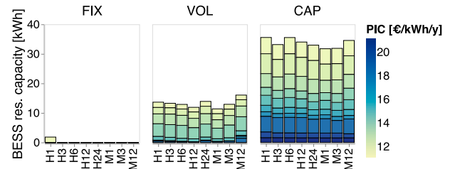
Fig. E.5. Sensitivity analysis results: installed individual consumer BESS capacities.
