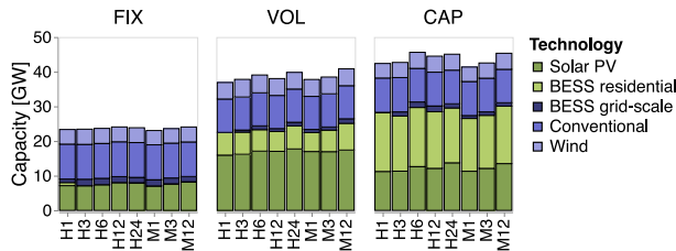
Fig. E.3. Sensitivity analysis results: generation capacity investments for all considered technologies.
