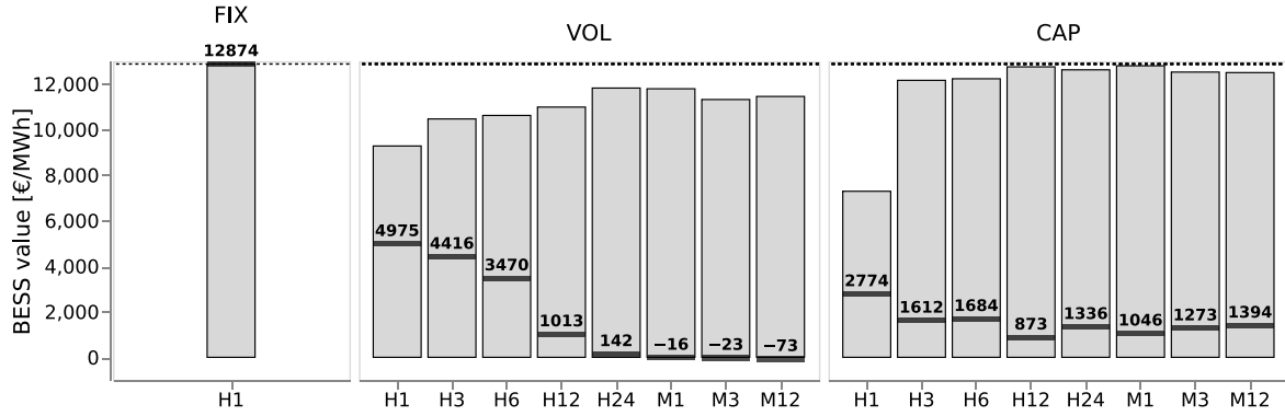
Fig. 6. Market value of residential BESS operations across decreasing temporal granularity of retail electricity prices and tariff types. Benchmark market values depicted by gray bars and the realized market values depicted by horizontal black lines are both calculated by Eq. (30). FIX: fixed tariff, VOL: volumetric tariff, CAP: capacity tariff, H: hourly temporal granularity, M: monthly temporal granularity.
