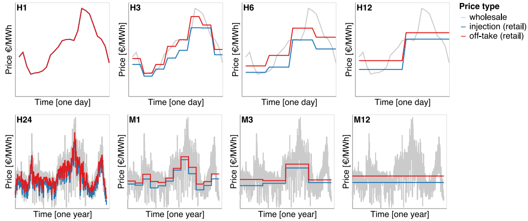
Fig. 2. Illustration of the temporal granularities for retail electricity prices considered in the study, from hourly (H1) pricing to yearly (M12). To better illustrate the price granularity in question, the x-axis either represents a day (H1–H12, top row) or one full year (H24 to M12, bottom row). Note that in H1 cases, wholesale, injection and offtake prices overlap.
