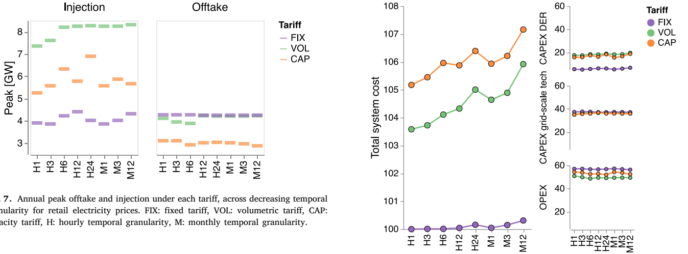
Fig. 8. Total system cost and constituents: CAPEX in DER, CAPEX in grid-scale technologies and OPEX. Costs are normalized using the lowest occurring total system cost: H1 FIX tariff total system cost. FIX: fixed tariff, VOL: volumetric tariff, CAP: capacity tariff, H: hourly temporal granularity, M: monthly temporal granularity.
