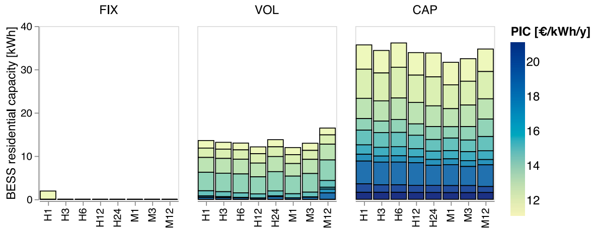
Fig. D.2. Installed consumer BESS capacities, under each tariff, across decreasing temporal granularity of retail electricity prices. Color scale indicates the perceived annualized investment cost (PIC). FIX: fixed tariff, VOL: volumetric tariff, CAP: capacity tariff, H: hourly temporal granularity, M: monthly temporal granularity.
