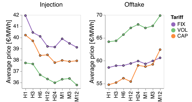
Fig. E.6. Sensitivity analysis results: Average offtake & injection prices.
