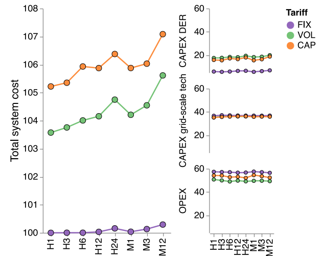
Fig. E.7. Total system cost and constituents. Costs are all normalized using the lowest occurring total system cost: H1 FIX tariff total system cost.
