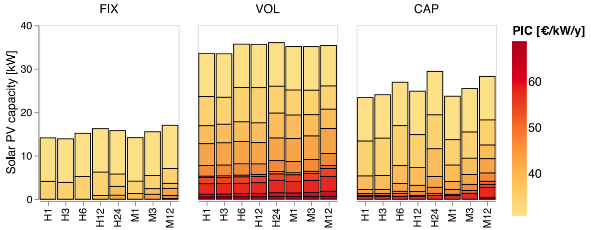
Fig. 4. Installed, individual, consumer solar PV capacities, under each tariff, across decreasing temporal granularity of retail electricity prices. Color scale indicates the perceived annualized investment cost (PIC) and each small block represents investment of each representative consumer. FIX: fixed tariff, VOL: volumetric tariff, CAP: capacity tariff, H: hourly temporal granularity, M: monthly temporal granularity.
