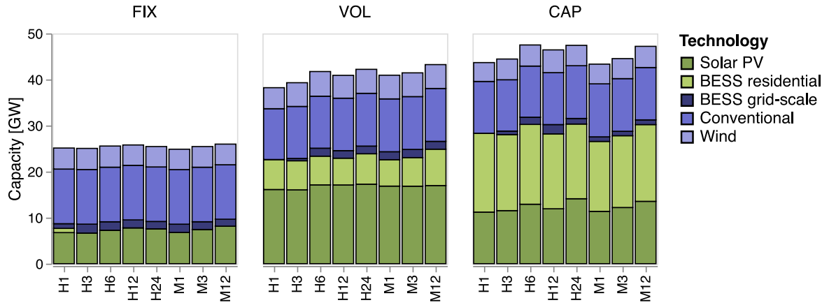
Fig. 3. Generation capacity investments for all considered technologies, under each tariff, across decreasing temporal granularity of retail electricity prices. The depicted solar PV and BESS capacities are the scaled, total capacities installed by all consumers. FIX: fixed tariff, VOL: volumetric tariff, CAP: capacity tariff, H: hourly temporal granularity, M: monthly temporal granularity.
