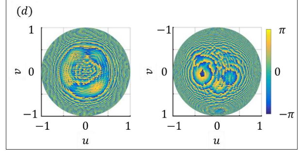
Fig.13 Normalized magnitude (a), (c) and phase (b), (d) of the y component of the PWS of the incident electric field for f_2 = 120\text{ GHz} when the terminal antenna is located in P_1 (a) and (b), or in P_2 (c) and (d). Top and bottom hemispheres are shown on the left and right, respectively.
