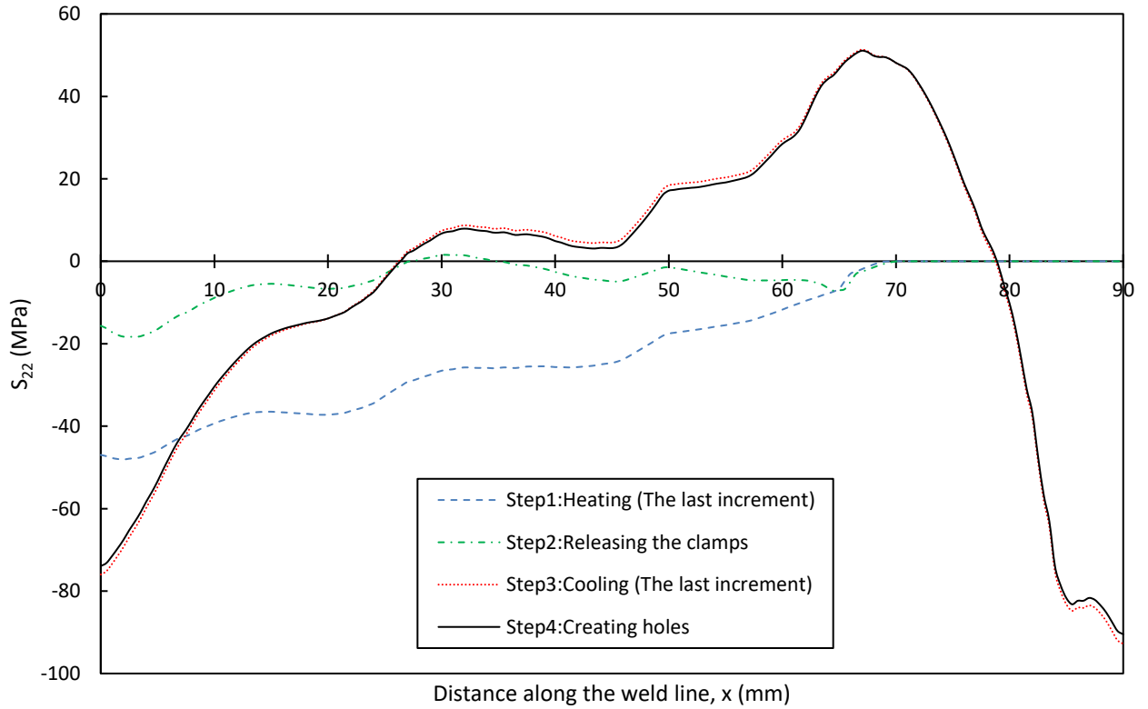
Fig. 14. Distribution of transverse stress on the front surface along the weld centerline, y = 0\text{mm} .
