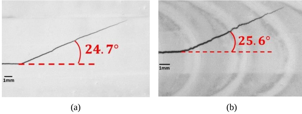
Fig. 5. Crack growth paths for loading angle \beta = 30^\circ in (a) non-welded specimen (b) welded specimen.
