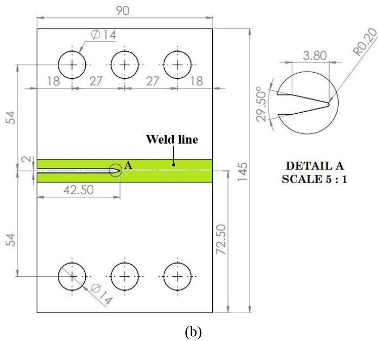
Fig. 2. Drawing of the (a) fixture and (b) CTS specimen, dimensions are in mm. (c) mixed mode fixture.
