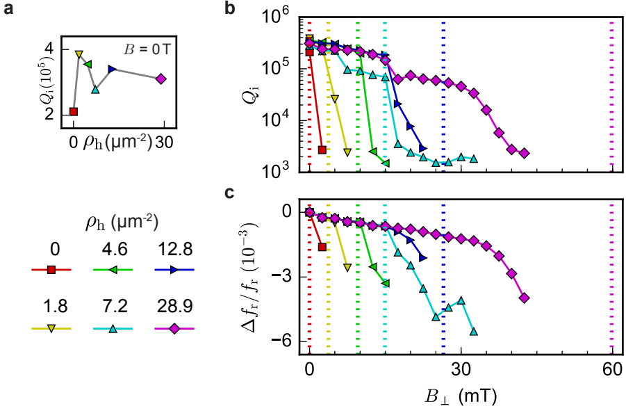
Figure 4.3: a Q_i versus \rho_h for field-cooled resonators at B_{\perp} = 0 T. b Q_i versus B_{\perp} for varying \rho_h . B_{\text{Th}} for each resonator is plotted with a colour matched vertical line. c \Delta f_r/f_r versus B_{\perp} for varying \rho_h with B_{\text{Th}} plotted as in b.
