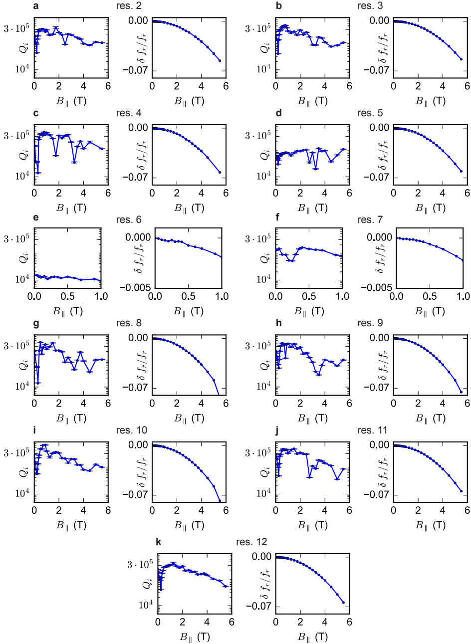
Figure 4.11: Resonators with holes in parallel magnetic field: from a to (k) the relative frequency shift ( \delta f_r/f_r(B) ) and Q_i(B) for resonators 2 to 12 in device 6. Resonators 6 and 7 could not be investigated above B = 1 T as their f_r overlapped.
