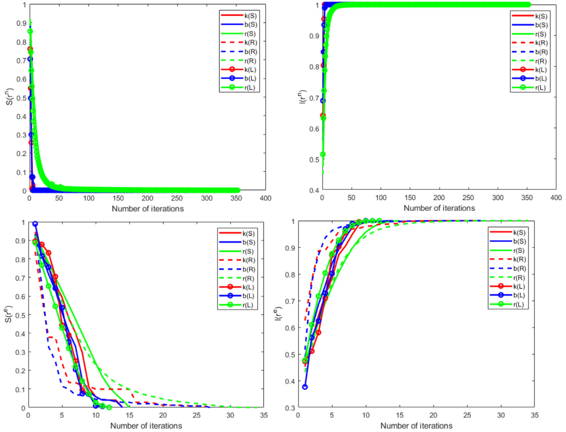
Fig. 7. Shanghai (S), Randstad (R) and London (L) performance under alternative node (above) and link (bottom) removal strategies (k – node centrality; b – betweenness centrality; r – random) with service line closures in terms of Relative Size, S , (left) and Average Normalized Shortest Path, l , (right).
