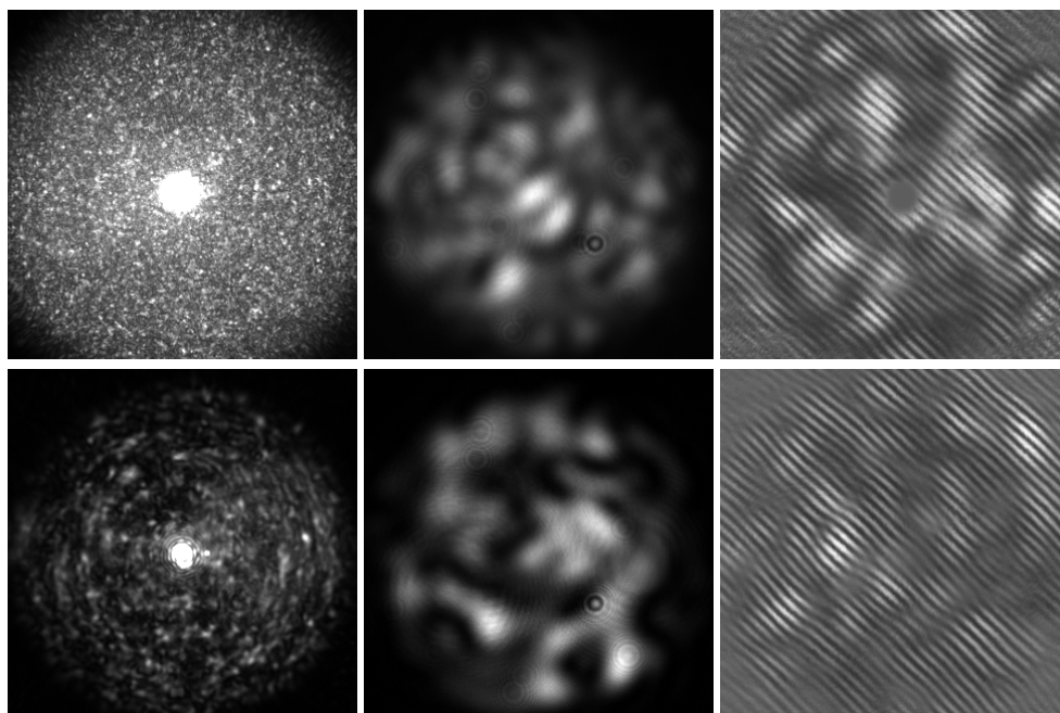
Fig. 5. Fringe and speckle patterns recorded from back-scattered light off the scattering beads solution (top) and off the spheroid sample (bottom). These images were observed by the WFS camera at the back aperture plane. The left images were obtained without a confocal pinhole, while the center and right images were taken with one in place. Additionally, the right images were flatfield corrected and interfered with the reference beam to produce fringes. The scattering bead solution shows a strong and homogeneous speckle pattern, while the spheroid shows larger speckles, indicating it is less scattering. The speckle pattern is spatially filtered by the confocal pinhole such that the fringe pattern contrast is enhanced, although larger-scale amplitude variations were still present. As can be seen in the center and right columns, the spatial frequency of the filtered speckles is similar for both samples. The fringe pattern has a higher spatial frequency than imposed by the confocal pinhole because the reference beam is introduced after the pinhole. All images were taken with the 20 \times objective and all fields of view are the same.
