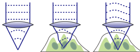
Fig. 1. Left : without sample, a plane wave focusses into a diffraction limited spot. Centre : in the presence of a perturbing sample, the focus is distorted leading to loss of signal and resolution. Right : using adaptive optics to pre-aberrate the wavefront, the focus can be improved.
