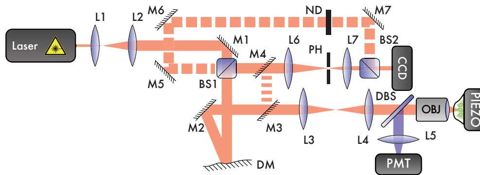
Fig. 2. Schematic optical setup showing the coherence-gated wavefront sensing principle. The pulsed laser beam is expanded (L1, L2) and then split (BS1) into a reference (long dashed) and a sample (solid) beam. In the sample beam the deformable mirror (DM) is re-imaged onto the objective's back aperture (L3, L4). The sample is mounted on an XYZ piezo stage, and the fluorescence signal is separated by a dichroic beam splitter (DBS) and detected by a photomultiplier tube. The back-reflected light in the sample beam is again reflected by the DM and directed into the wavefront sensor (WFS) by BS1, where the back aperture is re-imaged onto the CCD (L6, L7), after being spatially filtered by the pinhole (PH). The reference beam's optical path length and intensity are matched to that of the sample beam. The beams are combined on the CCD (BS2) where the temporally overlapping laser pulses interfere. By tilting folding mirrors in the reference beam (M6, M7) we tune the carrier frequency of the fringe pattern. Mirrors M3 and M4 are optional and are used to measure the influence of the DM for calibration purposes.
