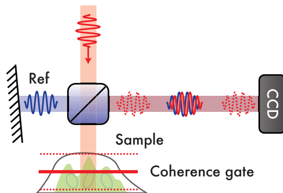
Fig. 3. Excitation light entering from above is split into a reference and sample beam. In the sample, the light is reflected at different depths, but only back-scattered light from a thin layer, the coherence gate (solid red), has the same optical path length as the reference beam and will interfere to form fringes on the CCD. Pulses that originate from deeper or shallower in the sample (dashed red lines) arrive later or earlier (dashed red waves) than the reference pulse and do not contribute to the fringe pattern and add a static background.
