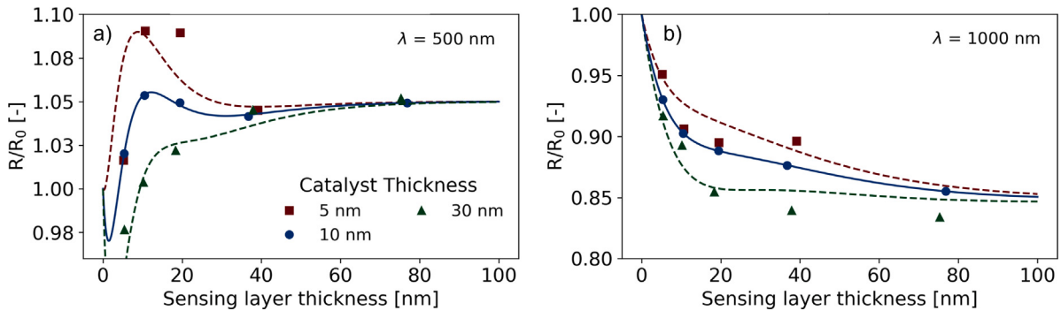
Fig. 13. Optical contrast upon hydrogen concentration from 0 of 4% for (a) \lambda = 500 nm and (b) \lambda = 1000 nm of the sensing stacks consisting of a 4 nm Ti adhesion layer, a d_{sens} thick Ta_{0.88}Pd_{0.12} sensing layer and for the Pd_{0.6}Au_{0.4} capping layer thicknesses indicated. The films all have a 30 nm PTFE layer. The continuous lines are the modeled data based on fitting the data of Fig. 12 with parameters presented in 1.
