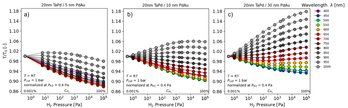
Fig. 9. Optical transmission as a function of the partial hydrogen pressure normalized to the transmission at P_{H_2} = 0.4 Pa. ('PTI diagrams') of 3 different samples with a 3 nm Ti, 20 nm \text{Ta}_{0.88}\text{Pd}_{0.12} sensing layers and a (a) 5 nm, (b) 10 nm and (c) 30 nm \text{Pd}_{0.6}\text{Au}_{0.4} capping layer. All samples have a 30 nm PTFE polymer coating and have been measured at 1 bar and room temperature for at partial hydrogen pressures ranging from 0.4 Pa to 10^5 Pa, i.e. corresponding to 0.0004\% \leq C_{H_2} \leq 100\% . The wavelengths are binned in groups of 50 nm.
