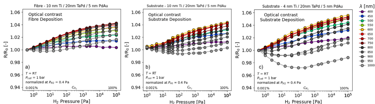
Fig. 15. PRI diagrams of the optical contrast in reflection for two sensing stack configurations at partial hydrogen pressures ranging from 0.4 Pa to 10^5 Pa measured at 1 bar at room temperature, binned per 50 nm with regard to wavelength of the signal for (a) a micro-mirror fiber with a 10 nm Ti - 20 nm Ta 0.88 Pd 0.12 - 5 nm Pd 0.60 Au 0.40 sensing stack deposited on the tip of the optical fiber, (b) 10 nm Ti - 20 nm Ta 0.88 Pd 0.12 - 5 nm Pd 0.60 Au 0.40 deposited on a substrate and (c) 4 nm Ti - 20 nm Ta 0.88 Pd 0.12 - 5 nm Pd 0.60 Au 0.40 deposited on a substrate.
