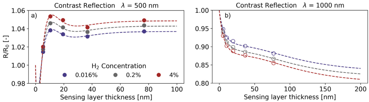
Fig. 12. Fits of the model as presented in Eq. (5) to the experimental optical contrast data in reflection of the 4 nm Ti adhesion layer - d_{sens} Ta_{0.88}Pd_{0.12} sensing layer and 10 nm Pd_{0.6}Au_{0.4} capping layer capped with 30 nm PTFE. The optical contrast is provided upon hydrogen concentration steps from 0 to 0.016%, 0.2% and 4% H_2 . The fits are made for both (a) \lambda = 500 nm light and (b) \lambda = 1000 nm light with parameters presented in 1.
