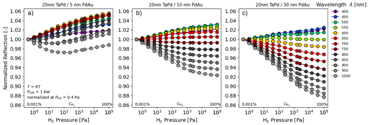
Fig. 8. Optical reflectivity as a function of the partial hydrogen pressure normalized to the reflectivity at P_{H_2} = 0.4 Pa. ('PRI diagrams') of 3 different samples with a 3 nm Ti, 20 nm \text{Ta}_{0.88}\text{Pd}_{0.12} sensing layers and a (a) 5 nm, (b) 10 nm and (c) 30 nm \text{Pd}_{0.6}\text{Au}_{0.4} capping layer. All samples have a 30 nm PTFE polymer coating and have been measured at 1 bar and room temperature for at partial hydrogen pressures ranging from 0.4 Pa to 10^5 Pa, i.e. corresponding to 0.0004\% \leq C_{H_2} \leq 100\% . The wavelengths are binned in groups of 50 nm.
