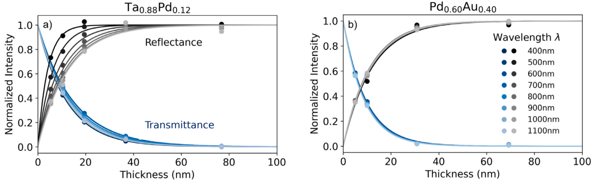
Fig. 10. Normalized reflectance and transmittance intensity of unloaded materials at different thickness for different wavelengths. The reflection data is measured at an 30^\circ angle and the transmission perpendicular to the samples. (a) \text{Ta}_{0.88}\text{Pd}_{0.12} , (b) \text{Pd}_{0.60}\text{Au}_{0.40} , the solid line display a fit to the data.
