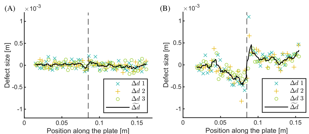
FIGURE 11 Measured defects of the plates pressed at 0.07 MPa in (A) and 3.5 MPa in (B). \Delta d is the deviation between tow spacing and mean tow spacing, measured along three different lines. \bar{\Delta d} is the moving average of the single measurement points, which is defined in this study as the defect size. The dotted lines indicate the thickness change in the middle of the plate.
