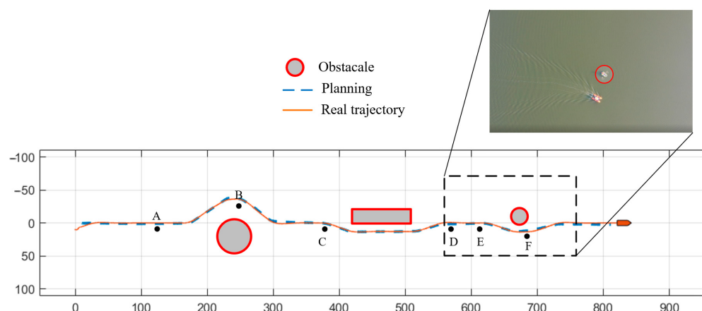
Figure 13. The performance of the vessel's sailing with static obstacles (Scenario 1).
