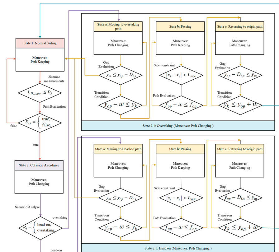
Figure 6. Conditional state machine of sailing.
