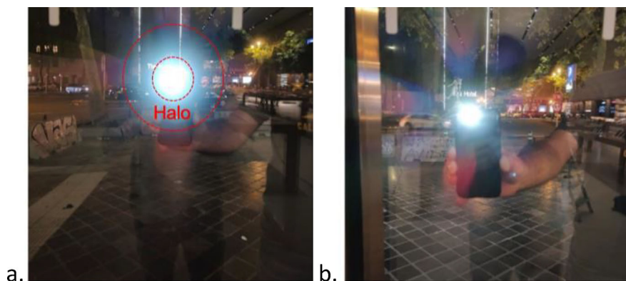
Fig. 2 Halo effect induced by the light scattering of a non-collimated light shining on the glazing between the light source and the observer: a Halo effect in glazing with haze visual defects; b lack of halo effect in a glazing without the haze visual defect
