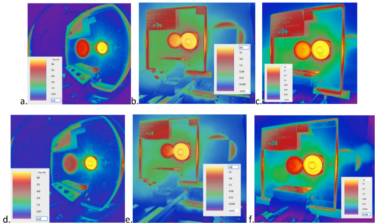
Fig. 9 False colour images of the luminance maps produced by means of HDR imaging. a Test condition “C”, largest distance and maximum light intensity for sample with 0.94% haze; b Test condition “B” medium distance and medium light intensity for sample with 0.94% haze; c Test condition “A”, largest distance and maximum light intensity for sample with 0.94% haze; d Test condition “C”, largest distance and maximum light intensity for sample with 0.28% haze; e Test condition “B” medium distance and medium light intensity for sample with 0.28% haze; f Test condition “A”, largest distance and maximum light intensity for sample with 0.28% haze;
