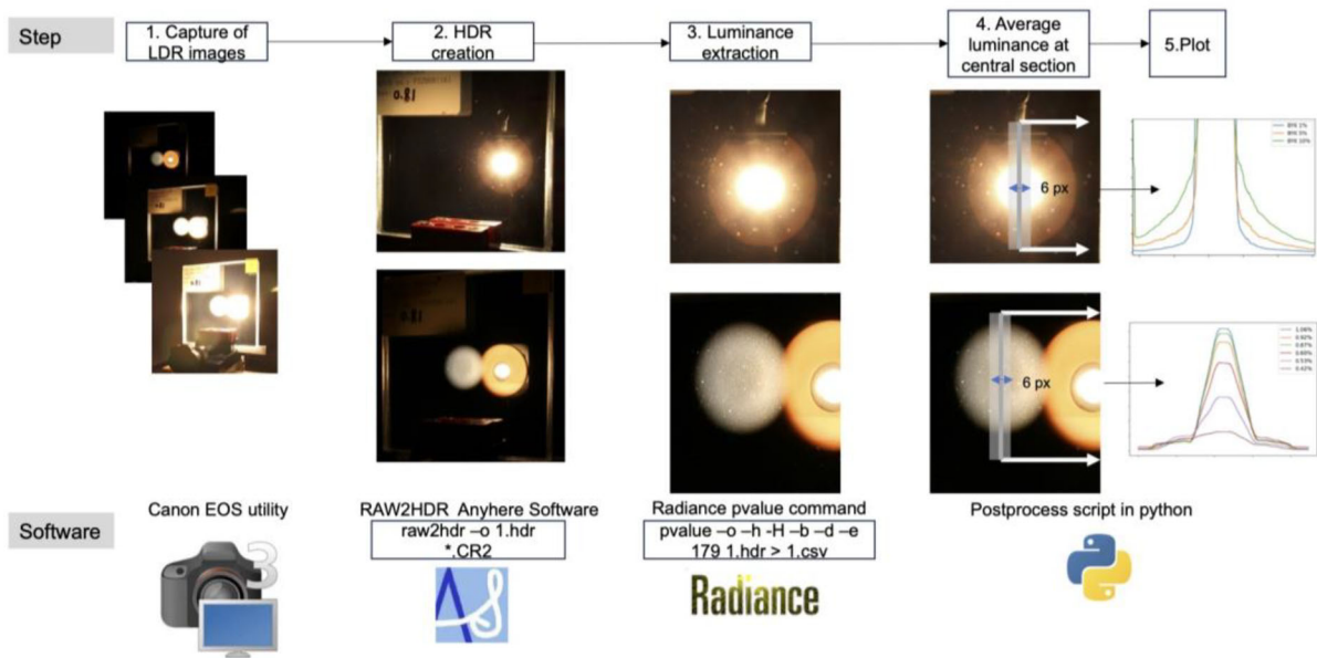
Fig. 6 Workflow to extract luminance values of the halo effect
