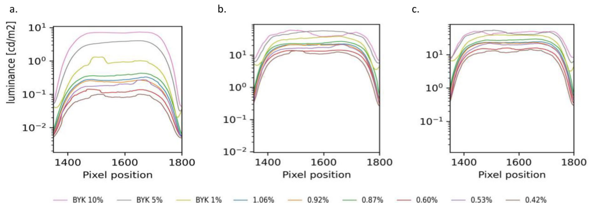
Fig. 7 Luminance values measured in proximity of the halo, for three different light intensity settings. a Test condition “C”, largest distance and minimum light intensity; b Test condition “B” largest distance and medium light intensity; c Test condition “A”, largest distance and maximum light intensity
