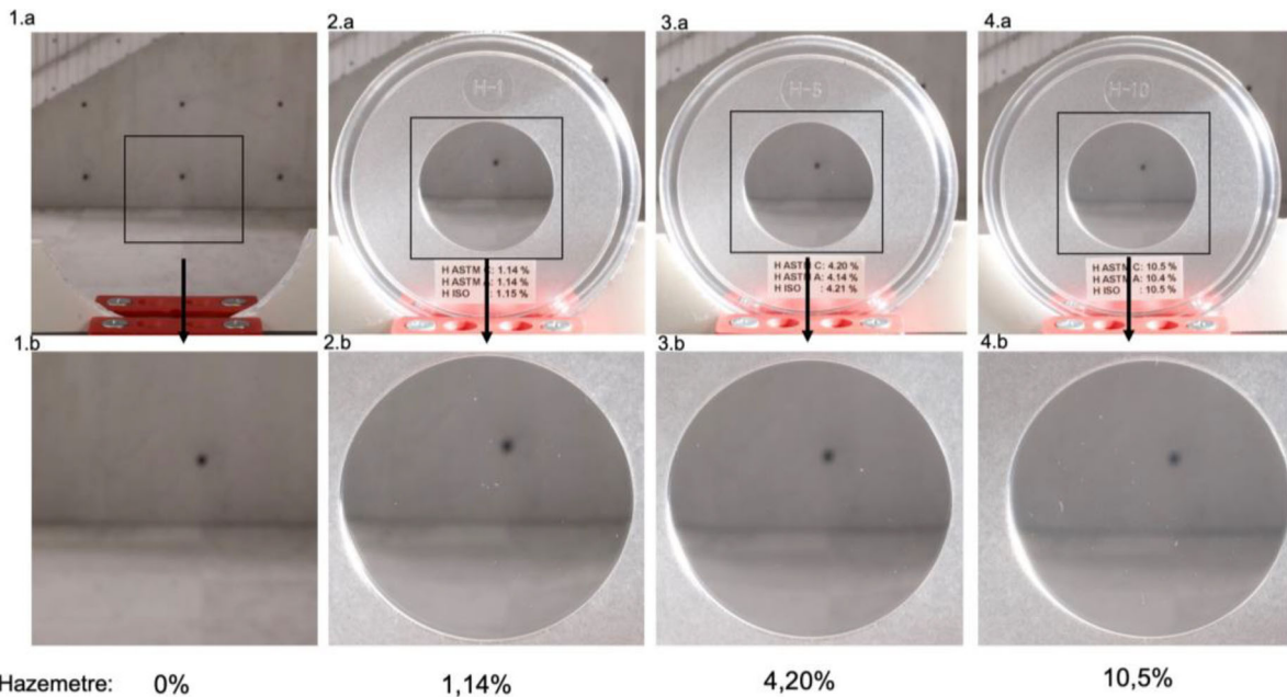
Fig. 4 Calibrated plastic samples with haze defect under under direct lateral lighting condition (1a, 2a, 3a, 4a) and zoomed image of the specimen (second row: 1b, 2b, 3b and 4b)
