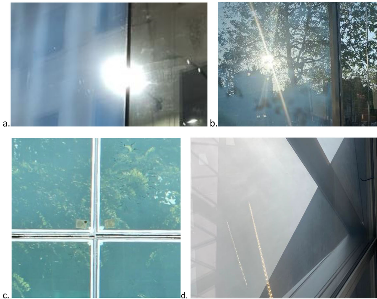
Fig. 1 Examples of visual defects related to view clarity in a few recent new façade and glazing assemblies: a haze defect due to interlayer performance at night under artificial lights; b haze defect under daylight conditions. c view clarity defect due to novel responsive electrochromic layers; d view clarity defect due to foginess in close cavity assemblies
