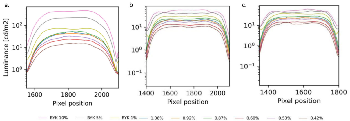
Fig. 8 Luminance values measured in proximity of the halo, for three different distances camera-sample. a Test condition “E”, closer distance and maximum intensity, b Test condition “D”, medium distance and maximum intensity; c Test condition “A”, further distance and maximum intensity
