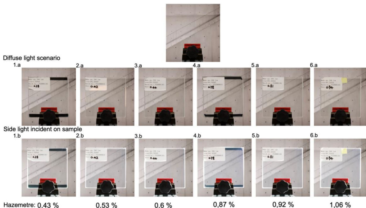
Fig. 3 Glazing samples used for the test with a progressive level of haze under indirect (first row: 1a, 2a, 3a, 4a, 5.1, 6a) and direct side lighting condition (second row: 1b, 2b, 3b, 4b, 5b, 6b). The image on the top is the view of the reference wall target behind the samples. The labels that are visible on the samples refer to a previous measurements by haze metre that was however re-done in later stage with higher accuracy
