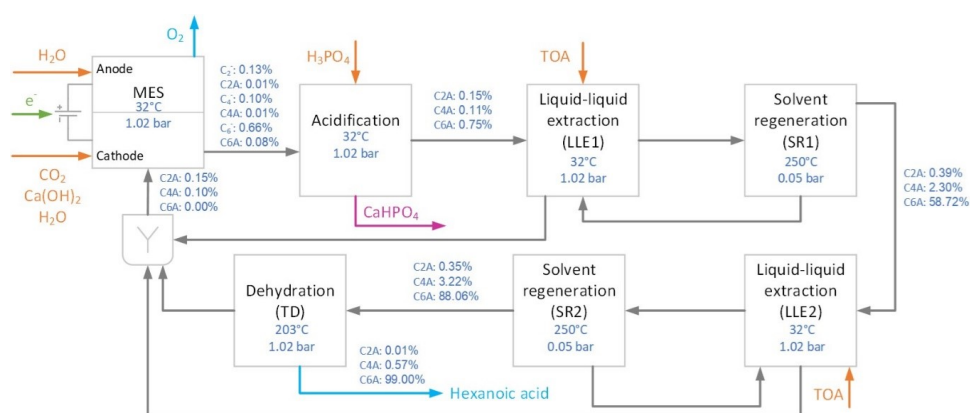
Fig. B1. Block flow diagram with operating conditions of key unit operations and mass purity of carboxylates and carboxylic acids of key streams, if any. MES: microbial electrosynthesis. LLE: liquid-liquid extraction. SR: solvent regeneration. TD: dehydration column. TOA: tri-octylamine. C 2 - : acetate. C 2 A: acetic acid. C 4 - : butyrate. C 4 A: butyric acid. C 6 - : hexanoate. C 6 A: hexanoic acid.
