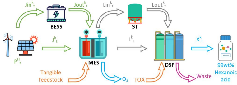
Fig. 4.2. A simplified illustration of the operating patterns of the MES plant. Notice: the acidification unit was omitted in this figure. DSP: downstream processing.
