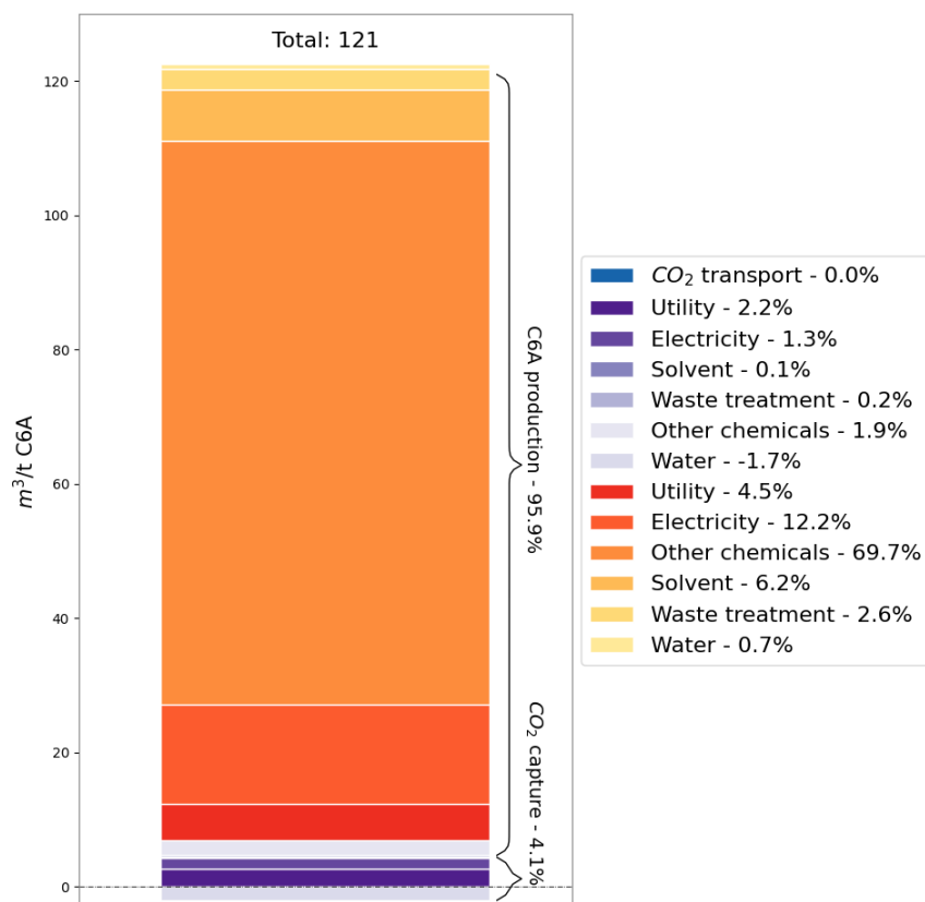
Fig. 5.7. Breakdown of water consumption of the MES route with economic allocation.
