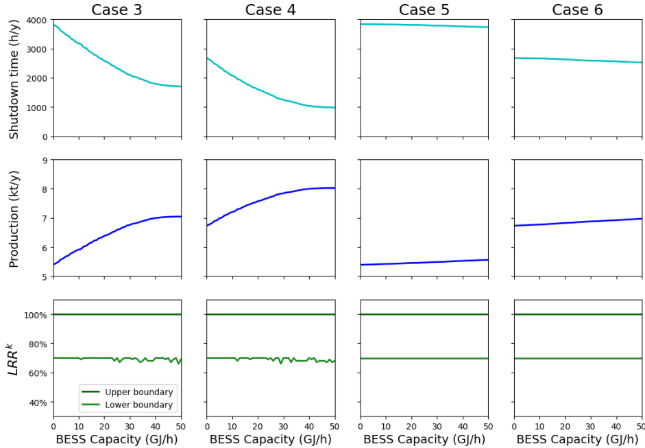
Fig. 3.4. Shutdown time, production quantity of hexanoic acid, and loss ratio range (LRR) in Cases 3 to 6.
