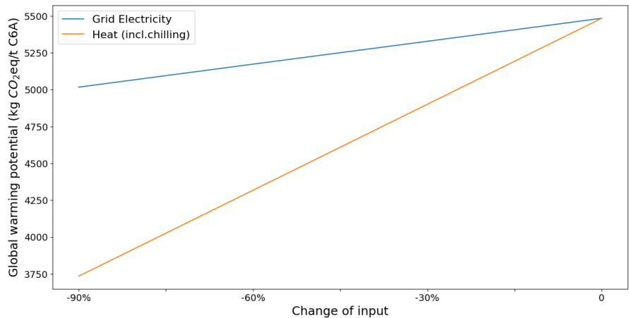
Fig. D1. Sensitivity analysis results - the impact of reduced carbon intensity of grid electricity and heat energy (incl. chilling) on the global warming potential per tonne hexanoic acid produced.
