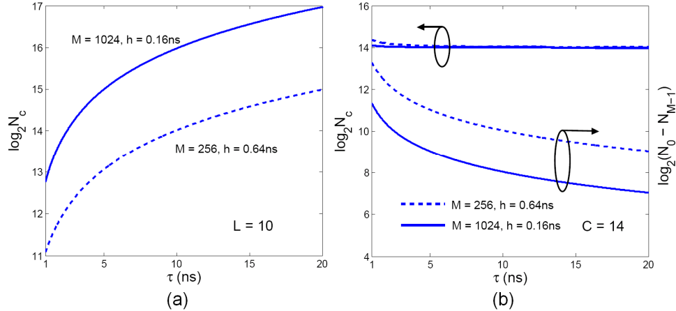
Fig. 6. Number of bits required to store N_c for (a) fixed accuracy mode and (b) fixed total count mode.
