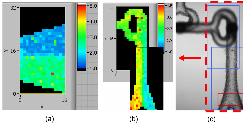
Fig. 8. Microfluidic mixing of fluorophore solutions. (a) Rhodamine B in water and ethanol (both 100 \mu M) come together at a junction at a high flow rate (50 \mu l/min). (b) Interface between the two streams (here 100 \mu M Rhodamine B and 20 \mu M Rhodamine 6G in water) dissolves as they mix along the channel. (c) Brightfield image of the microfluidic micromixer chip (Micronit Microfluidics, FC_TD26).
