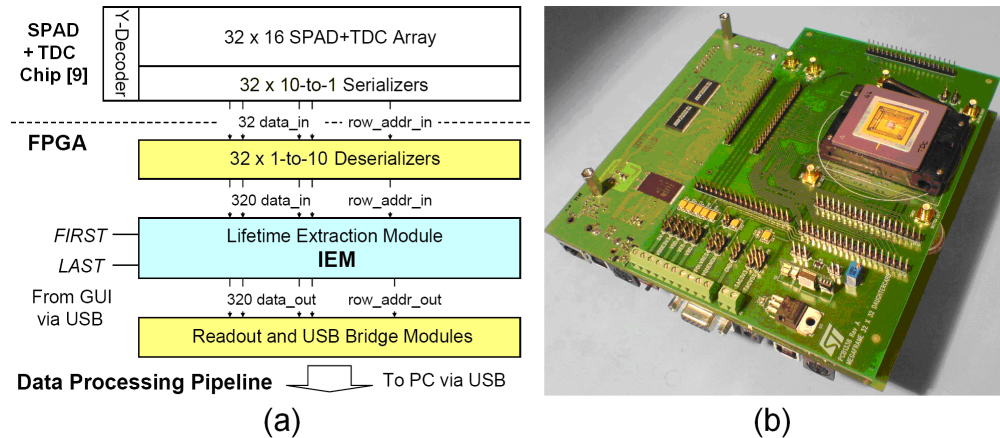
Fig. 5. (a) IEM FPGA implementation and data path (b) Imager assembly on an EPFL LASP motherboard.
