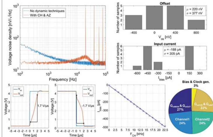
Figure 31.4.5: Voltage noise density vs frequency. Histogram of the offset voltage and input current for 15 Samples. Slew rate with a 4V input voltage step (0.2 to 4.2V) in a buffer configuration. Input current vs chopping frequency. Power breakdown.
