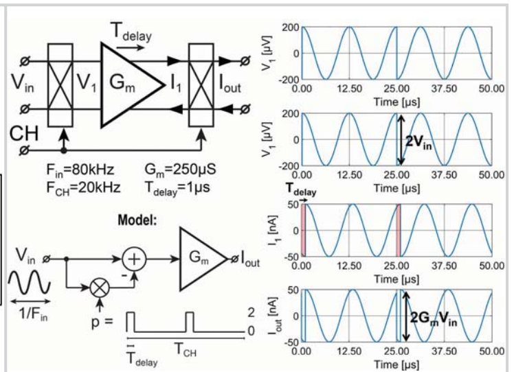
Figure 31.4.2: Chopped OTA with a delay (top left), and the resulting signals (right) when an input signal ( V_{in} ) is applied, showing large spikes at the output ( I_{out} ), and a model for the resulting waveform (bottom left).
