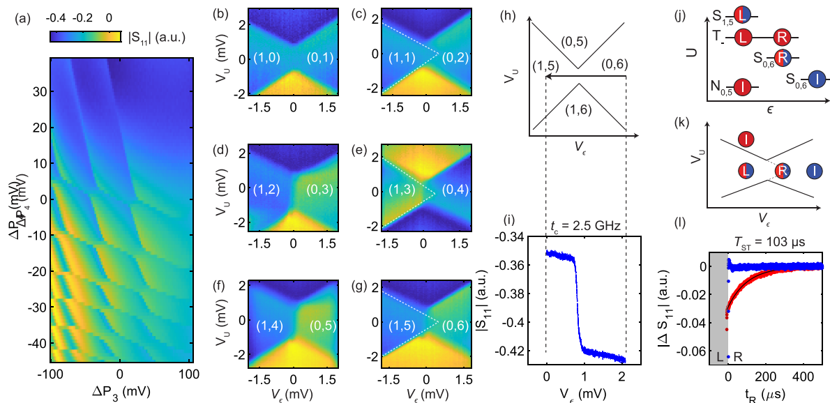
Figure 2. (a) Double quantum dot charge stability diagram obtained by rf-charge sensing in a reconfigurable quadruple quantum dot. A double quantum dot is formed under P_3 (blue) and P_4 (red) with controllable interdot tunnel coupling by tuning interdot barrier gate B_{34} and using rf-charge sensing we can clearly monitor the charge occupancy. The map is taken with 2000 averages. (b–g) Charge stability diagrams of charge anticrossings (1, N - 1) \leftrightarrow (0, N) for integer steps in N from 1 to 6. When N is odd (b,d,f), no spin blockade is present in the transitions. For even N (c,e,g), we observe spin blockade evidenced by triangular extensions of the charge addition lines (white lines are drawn in as a visual guide). (h,i) Interdot tunnel coupling measurement for the (1, 5) \leftrightarrow (0, 6) transition. Sweep direction is negative in detuning axis to avoid spin blockade artifacts in spectrum. A tunnel coupling of t_c = 2.5 GHz is obtained and kept within 200 MHz of this value for all measurements in the work. (j) Cartoon of the initialization (I), loading (L), and readout (R) points of our pulse sequences in detuning \epsilon and energy U space. The blue sequence loads the |S_{(1,5)}\rangle singlet state which is not blocked on readout. The red sequence initializes in the (0, 5) charge state N_{0,5} and loads a randomly oriented spin resulting in the singlet state or triplet state with equal probability (red), the latter of which results in a blocked signal. (k) Pulse sequences as a function of virtual detuning ( V_\epsilon ) and energy ( V_U ) gates for the case of loading a singlet state (blue) and triplet/singlet state with equal probability (red). (l) Readout traces showing the signal difference between the spin blocked (red) and unblocked (blue) signals as a function of time spent in the read phase ( t_R ). Each trace is averaged 1000 times. The small deviation in the blue trace around t_R = 0 \mu s is due to ringing in the applied AWG pulse. Loading a random spin under P_3 (red) leads to a singlet–triplet decay time of T_{ST} = 103 \mu s.
