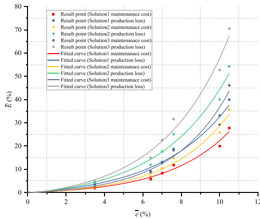
Fig. 12. Average Prediction Error \bar{e} versus maintenance performance.
