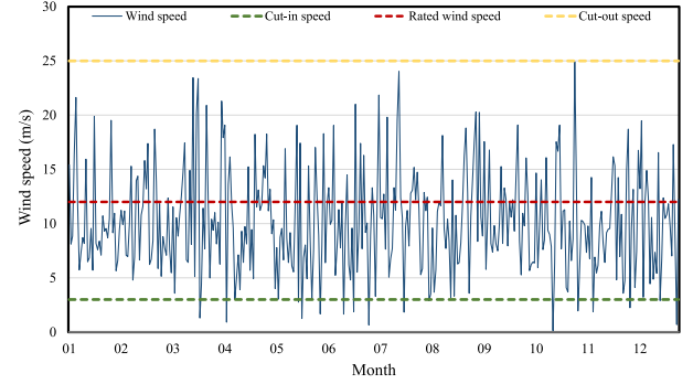
Fig. 8. Wind speed and turbine design parameter.
