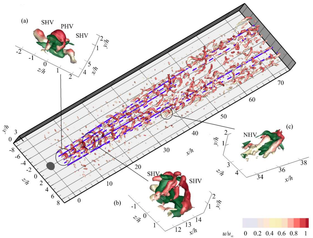
Fig. 11. The instantaneous flow pattern of the hemisphere wake visualized by the \lambda_2 criterion, color coded by u/u_\infty ; Solid and dash dot purple lines: clockwise and anti-clockwise rotating streamwise vortices; the ejection event shown with green iso-surface of u'v'/u_\infty^2 = -0.002 .
