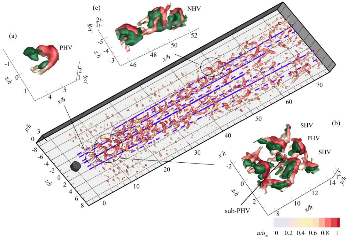
Fig. 8. The instantaneous flow pattern of the cylinder wake visualized by the \lambda_2 criterion, color coded by u/u_\infty ; Solid and dash dot purple lines: clockwise and anti-clockwise rotating streamwise vortices; the ejection event shown with green iso-surface of u'v'/u_\infty^2 = -0.002 .
