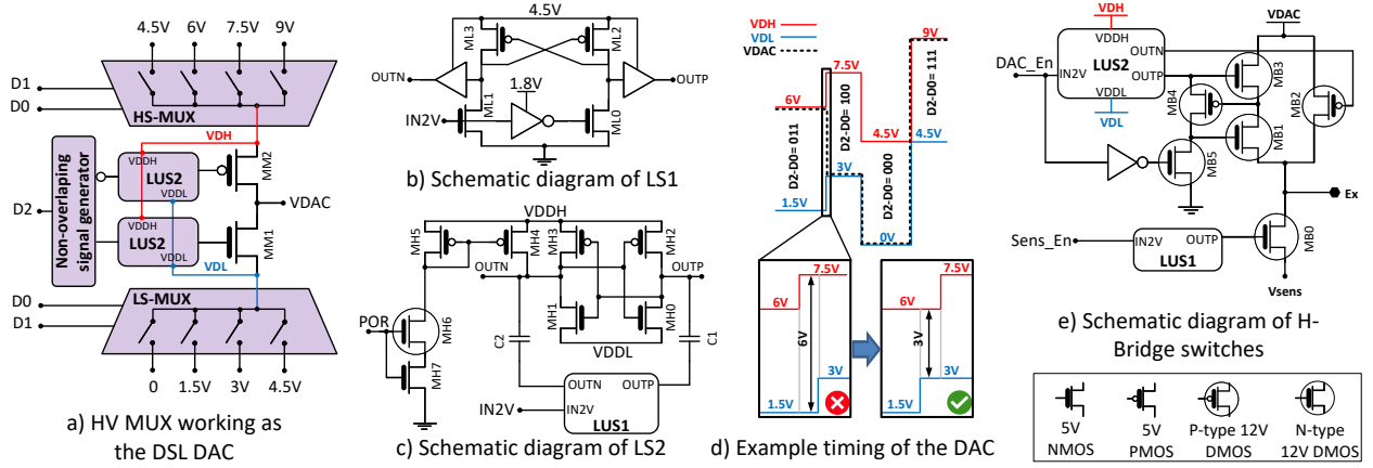
Fig. 4: Schematic and timing diagram of high-voltage DAC and H-bridge. The bulk of all the transistors in this figure are connected to their gates. An N+ buried layer is used for isolating the substrate of the NMOS devices when needed.
