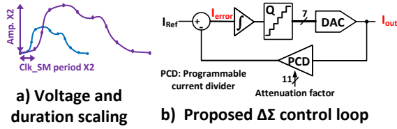
Fig. 2: Proposed a) scaling method b) Delta Sigma Loop.
