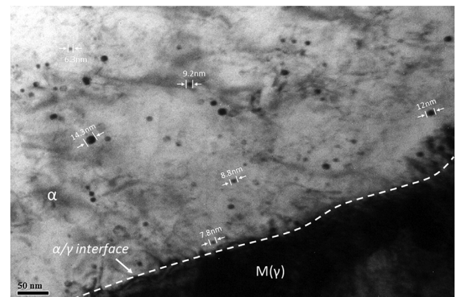
Fig. 13. TEM image showing carbide distribution near the \alpha/\gamma interface after a type H1 cycle.
