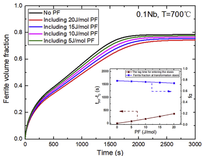
Fig. 14. The kinetics of the first \gamma \rightarrow \alpha transformation at 700^\circ\text{C} in the 0.1Nb alloy simulated by the GEB model. Inset summarizes the stasis ferrite fractions and the lag time for entering the transformation stasis predicted by the GEB model as a function of PF.
