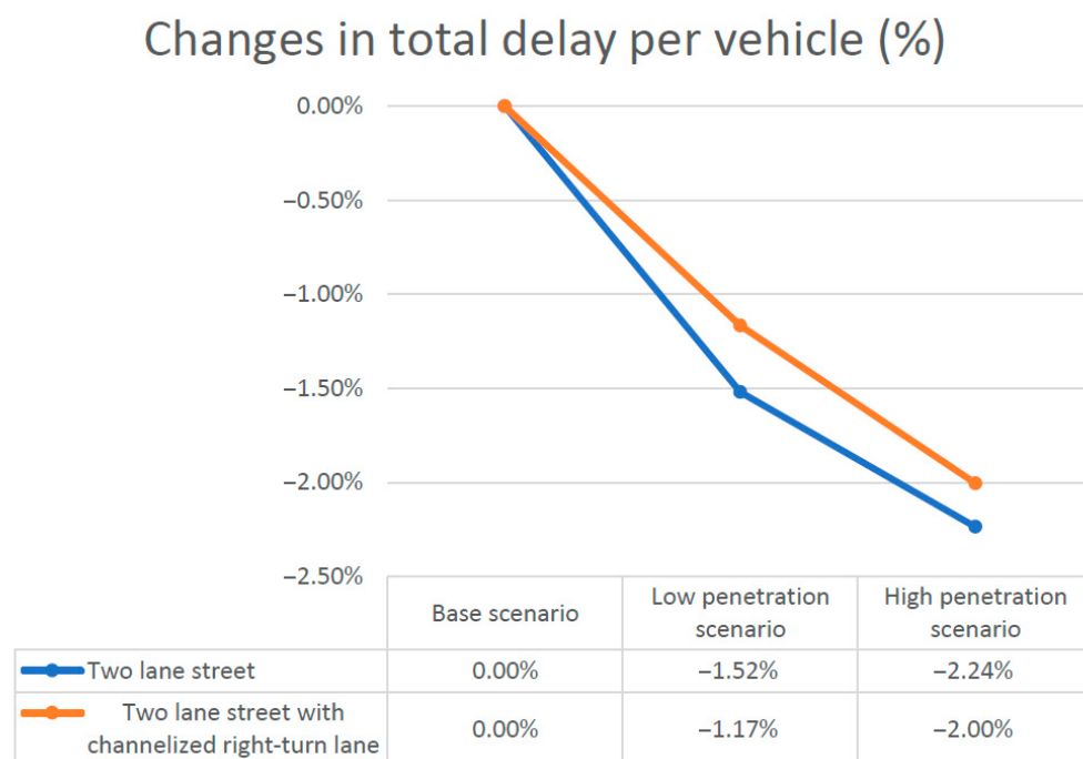
Figure 5. Changes in total delay per vehicle (%).
