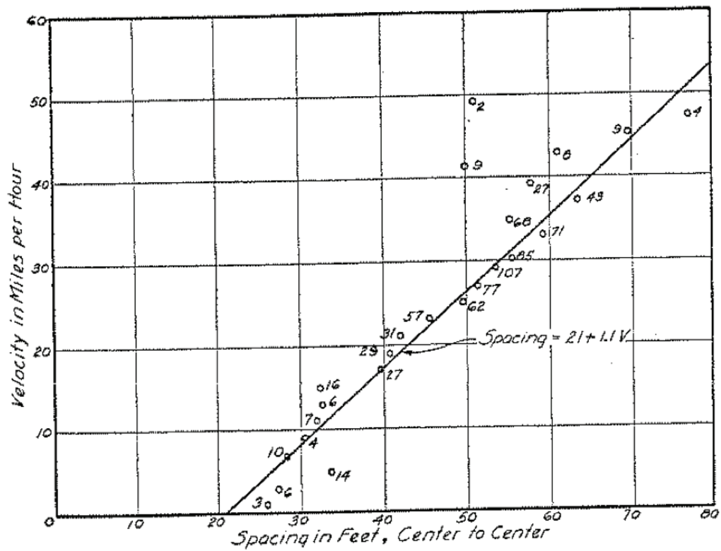
FIGURE 2 Greenshields' original fundamental diagram (1934), showing a linear relation between spacing and speed. Picture from [1].
