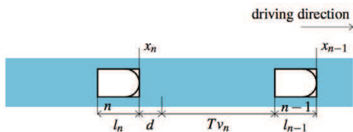
FIGURE 9 Variables and parameters in Pipes' safe distance model. The position x_n of the n -th vehicle is determined the position x_{n-1} of it leader and the safe distance between them. The safe distance is a constant distance determined by the distance at standstill d , the vehicle length l_{n-1} and a variable safe stopping distance Tv_n with T time safe time headway and v_n the speed.
