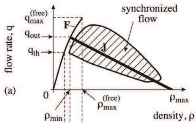
FIGURE 7 Fundamental diagram with infinitely many admissible states in the congestion branch (shaded area). Picture from [77]. For detailed explanation of the labels, we refer to [77].
