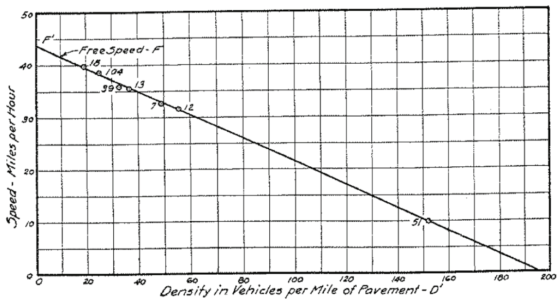
FIGURE 3 Greenshields' fundamental diagram (1935), showing a linear relation between density and speed. Picture from [4].
