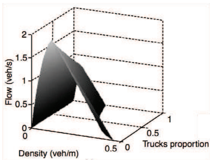
FIGURE 8 3 dimensional fundamental diagram where a high trucks proportion leads to lower speeds and flows. Picture from [13].
