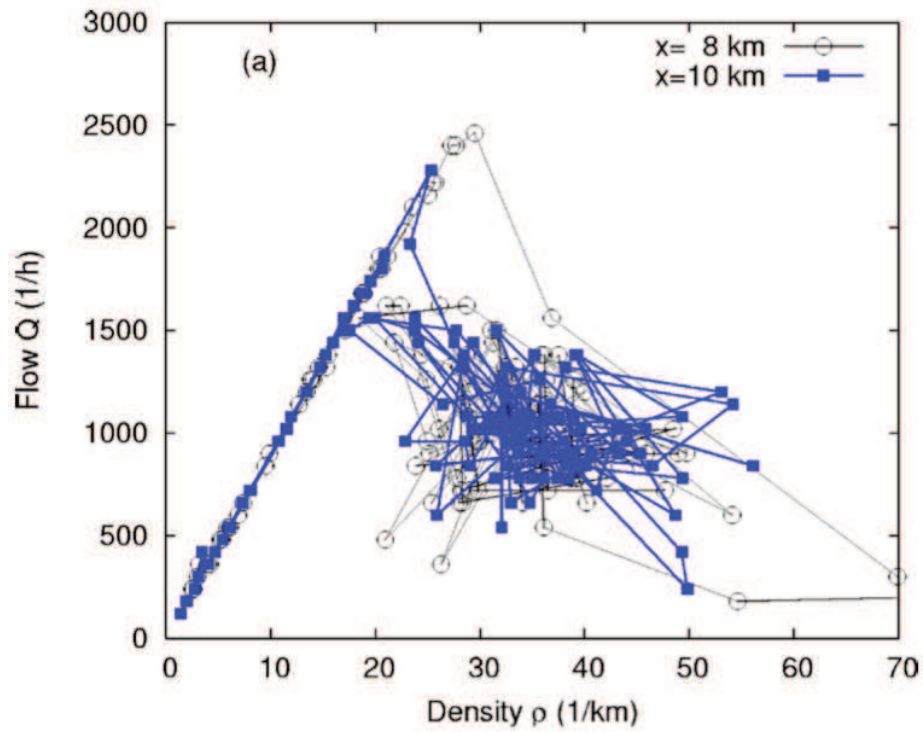
FIGURE 4 Scatter in an observed density-flow plot. Picture adapted from [76].
