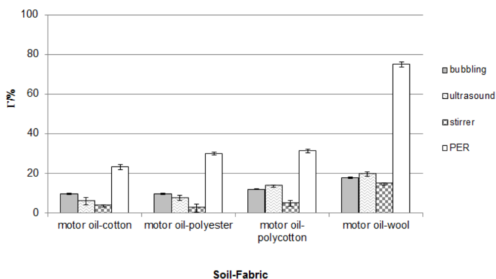
Figure 5.5: Influence of different types of mechanical action on cleanability with 1 L apparatus
