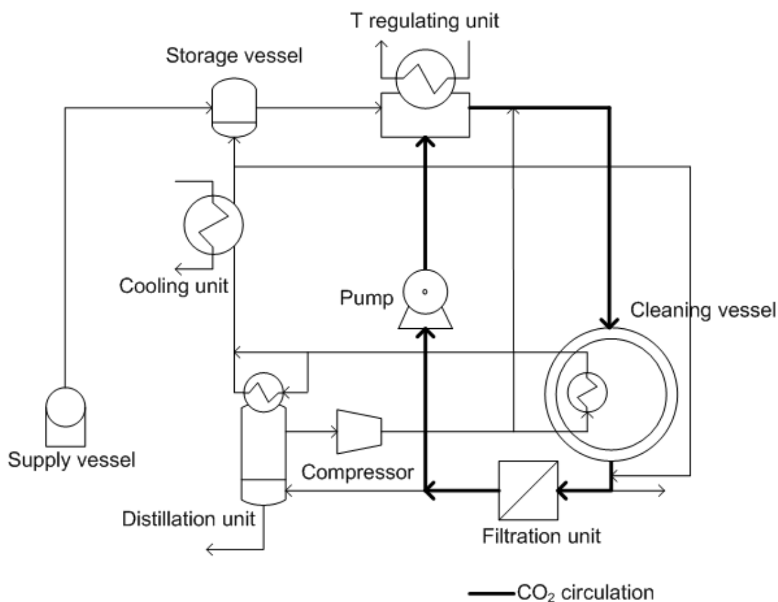
Figure 8.4: Flow diagram of the optimized CO 2 dry cleaning machine
