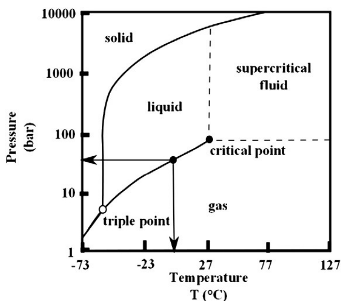
Figure 1.1: The P-T phase diagram of CO 2 . The black dot on the gas-liquid boundary line represents a possible condition in dry-cleaning (45 bar and 10°C), adapted from Leitner [8]
