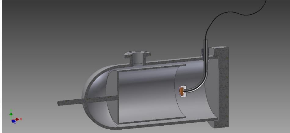
Figure 6.3: Endoscopic camera installation inside 25 L Delft apparatus with rotating drum
