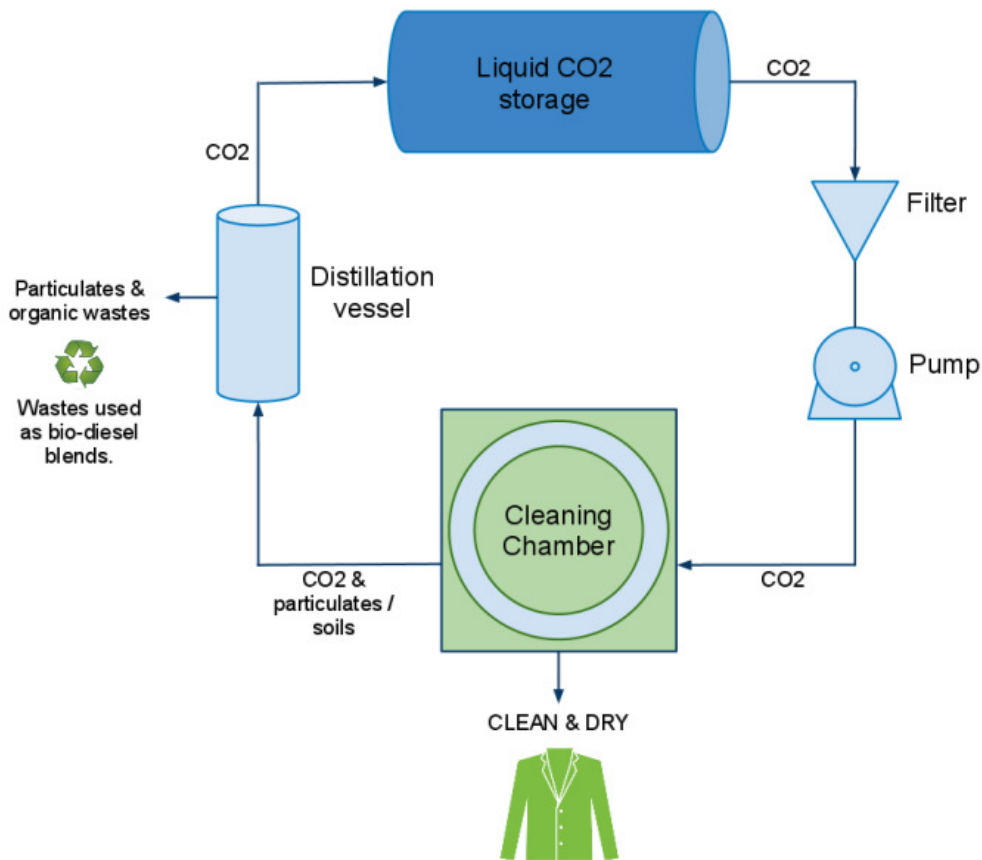
Figure 2.4: CO 2 Nexus process flow diagram
