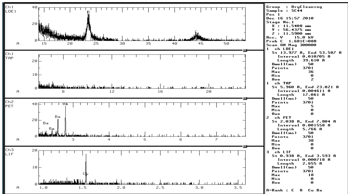
Figure 3.8: EMP graph for sebum colored with carbon black on cotton after washing
