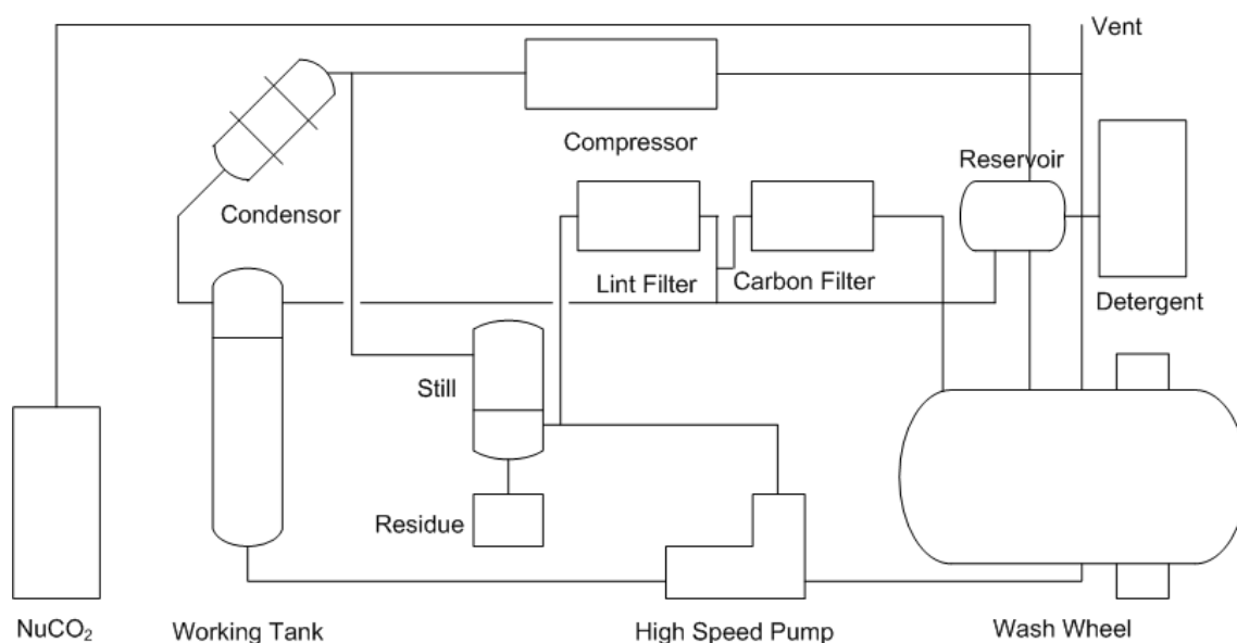
Figure 2.2: MICO process schematic unit [12]
