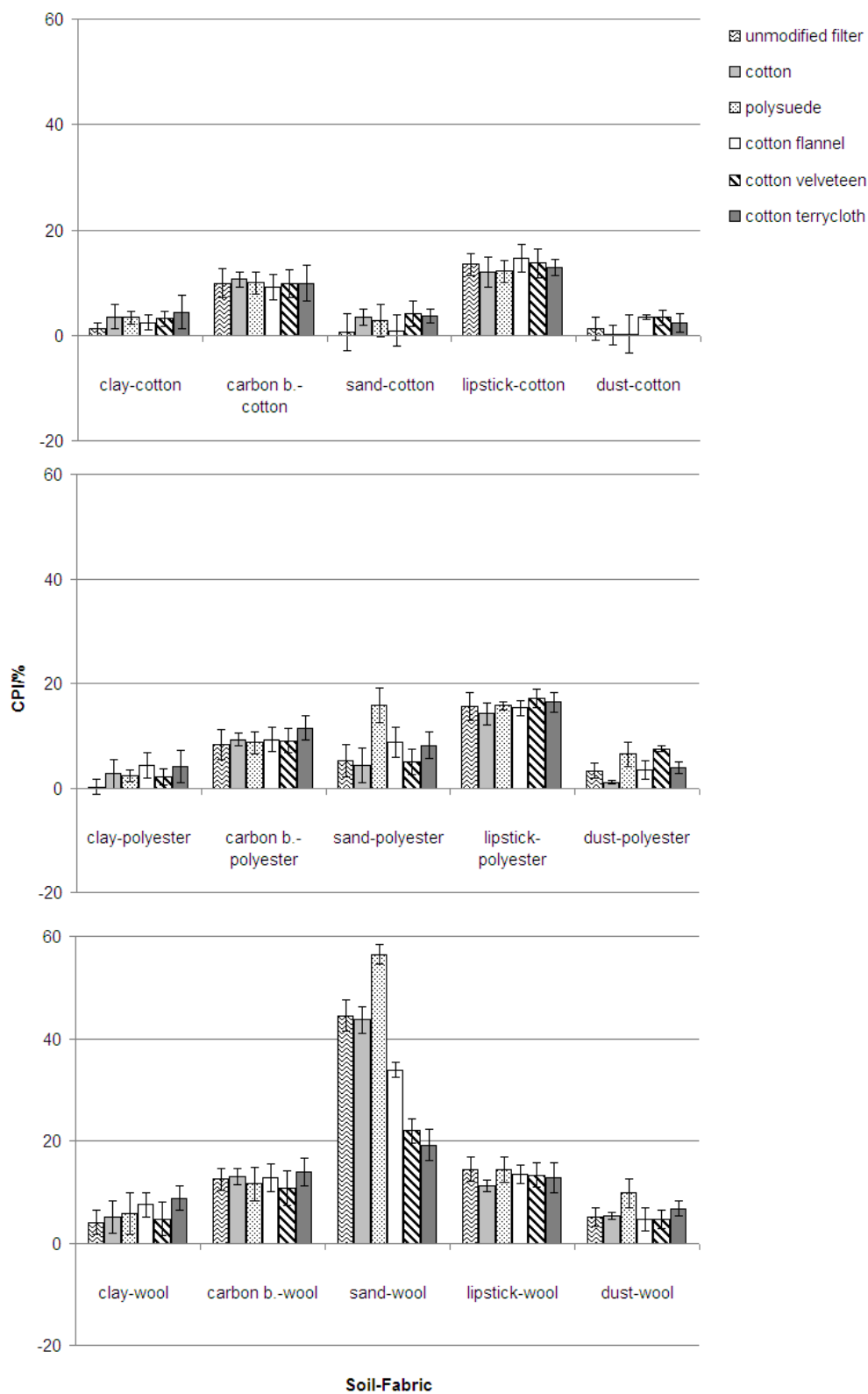
Figure 3.11: Influence of using different textile materials as second pre-filter on CPI
