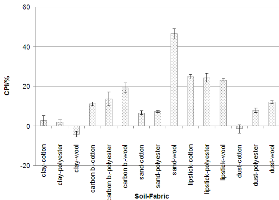
Figure 3.3: Cleaning result with different types of soil
