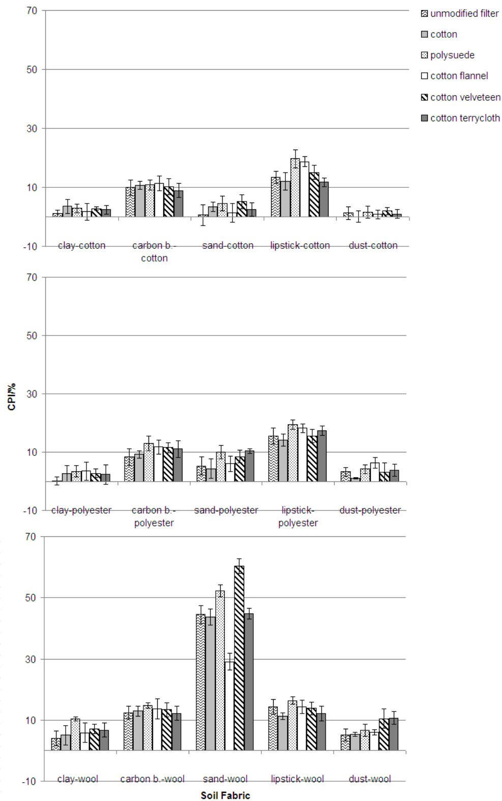
Figure 3.10: Influence of using different textile materials as pre-filter on CPI
