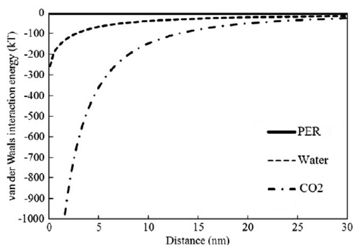
Figure 7.4: Van der Waals interaction energy between a model soil particle (silica radius 3 \mu\text{m} ) and model fabric (cellulose) in PER, water and CO 2 [9]
