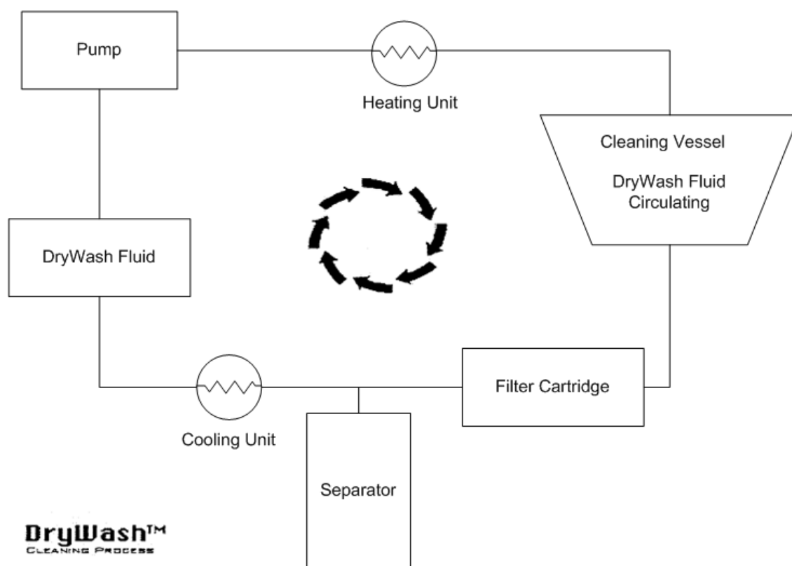
Figure 2.3: DryWash process schematic
