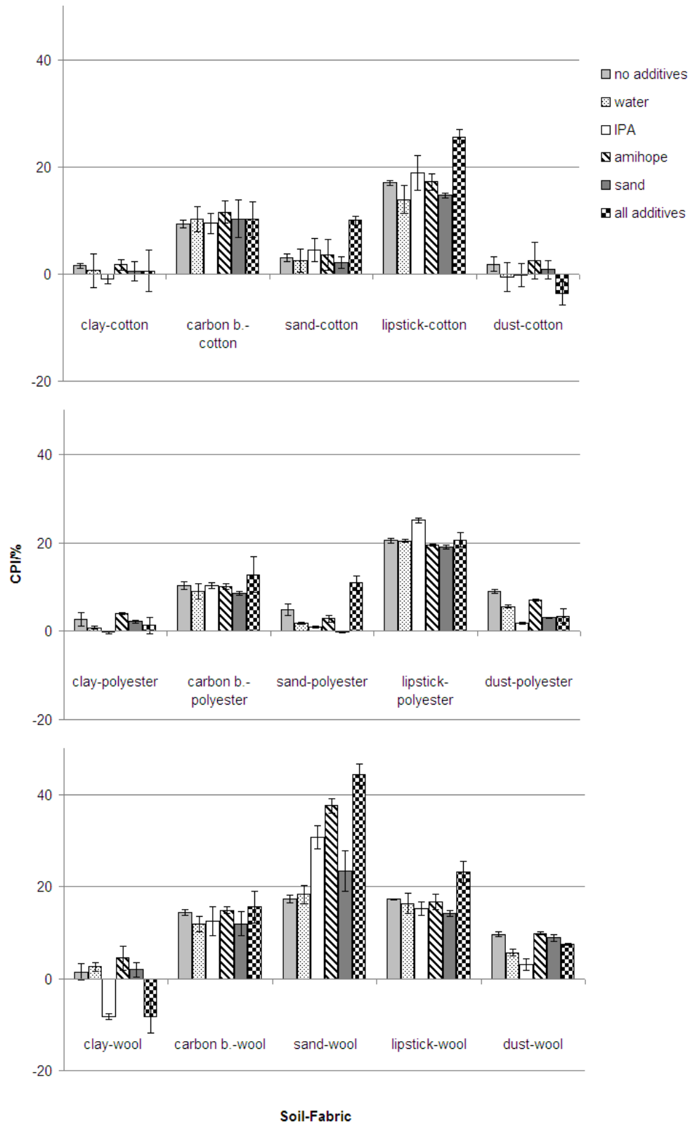
Figure 4.3: Influence of additive type on CPI for different types of soiled material
