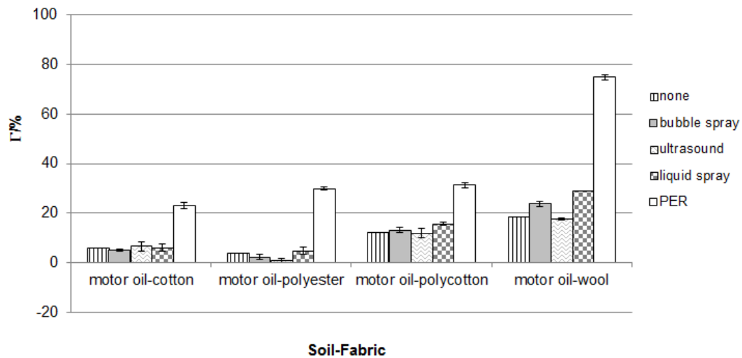
Figure 5.7: Influence of different mechanical actions on cleanability with 90 L apparatus
