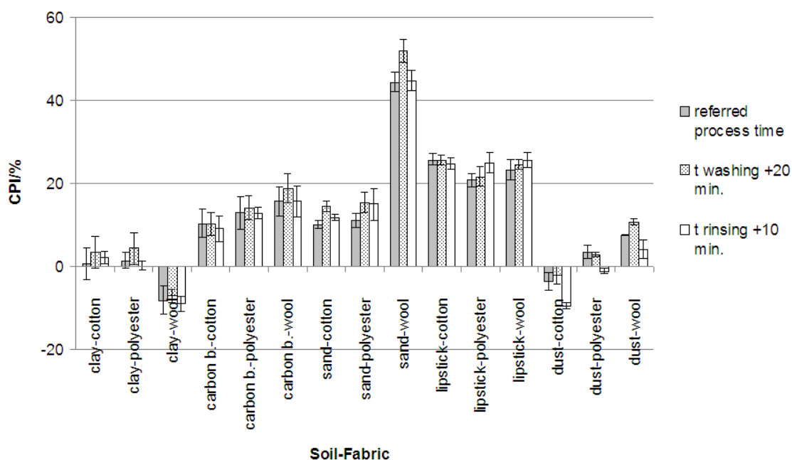
Figure 4.10: Influence of washing and rinsing time on CPI
