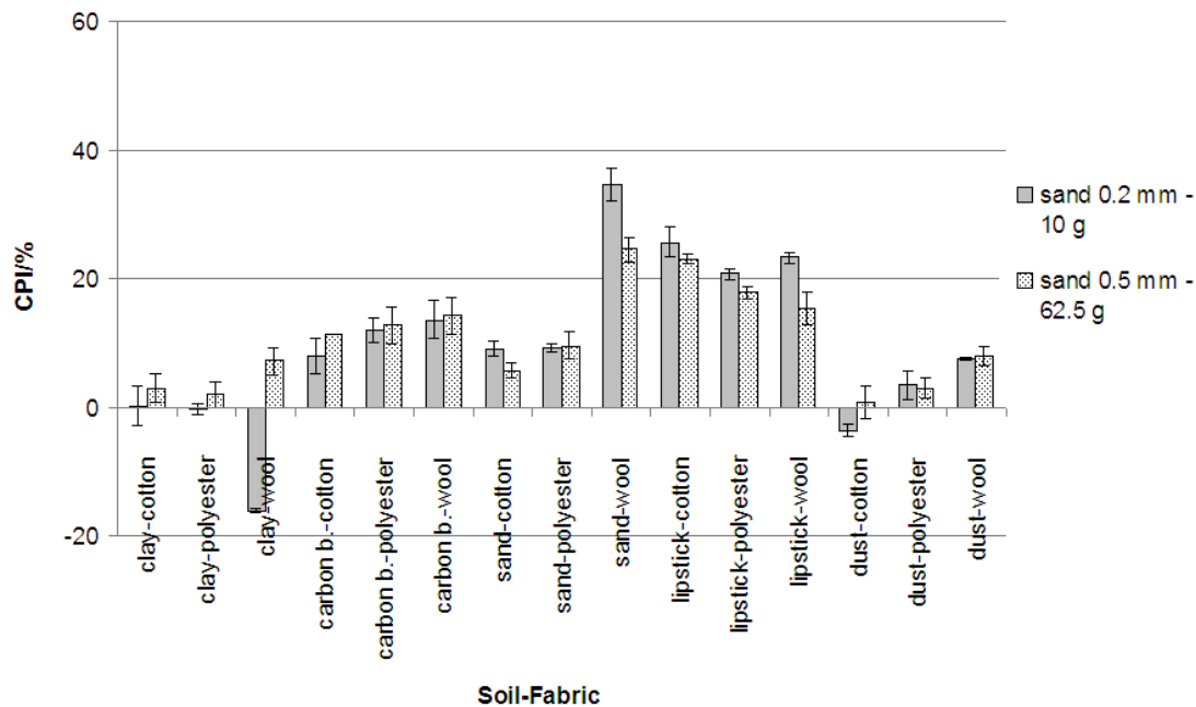
Figure 4.6: Influence of same specific surface area, different sand diameter on CPI
