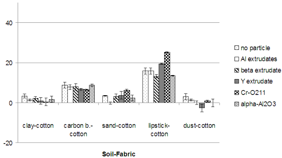
Figure 4.7: Influence of type of additional particles on CPI
