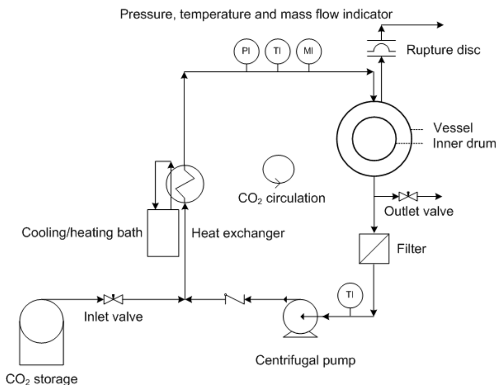
Figure 6.1: Schematic representation of 25 L Delft dry-cleaning apparatus
