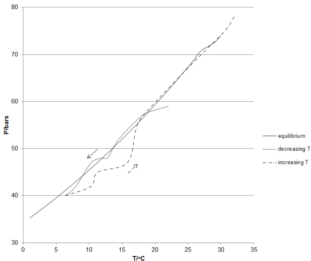
Figure 5.4: CO 2 L-V phase diagram during the observation of bubbling process at decreasing temperature from 23°C (room T) to 12°C, and then from 12°C to 7°C, followed by increasing temperature from 7°C to 12°C, and then 12°C to 33°C
