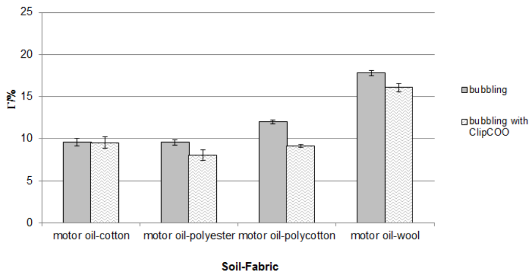
Figure 5.8: Influence of ClipCOO detergent on cleanability with 1 L apparatus
