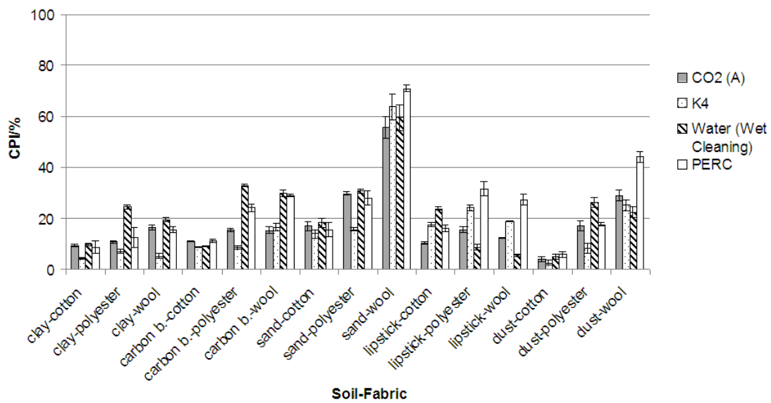
Figure 6.7: Cleaning Performance Index for different cleaning solvents
