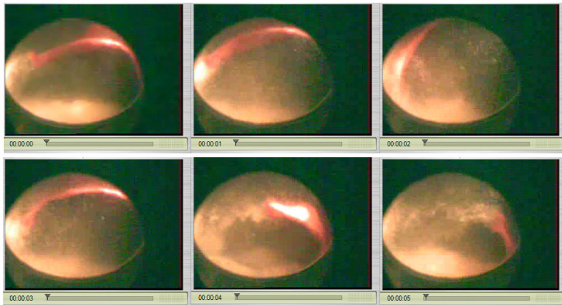
Figure 6.4: Textile movement inside a rotating drum for 1 piece of textile, rotation speed: 75 rpm, rotation direction: clockwise-counter clockwise, amount of CO 2 : 6 kg, T: 10°C, no pump circulation, no baffle
