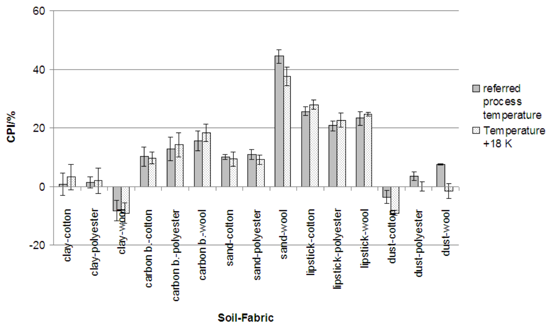
Figure 4.11: Influence of process temperature on CPI
