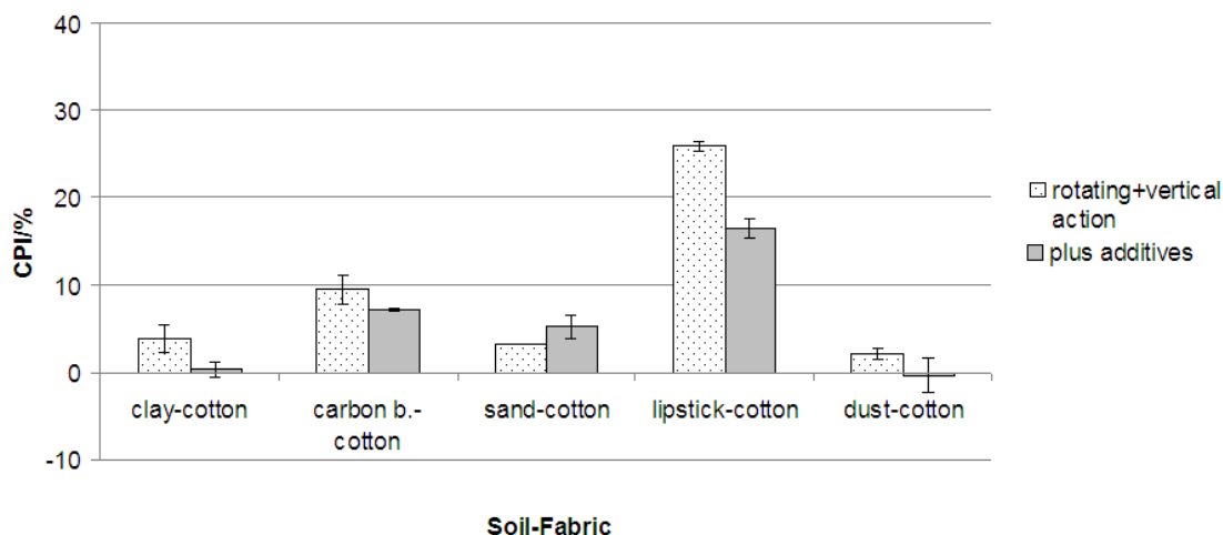
Figure 7.3: Cleaning Performance Index with and without additives
