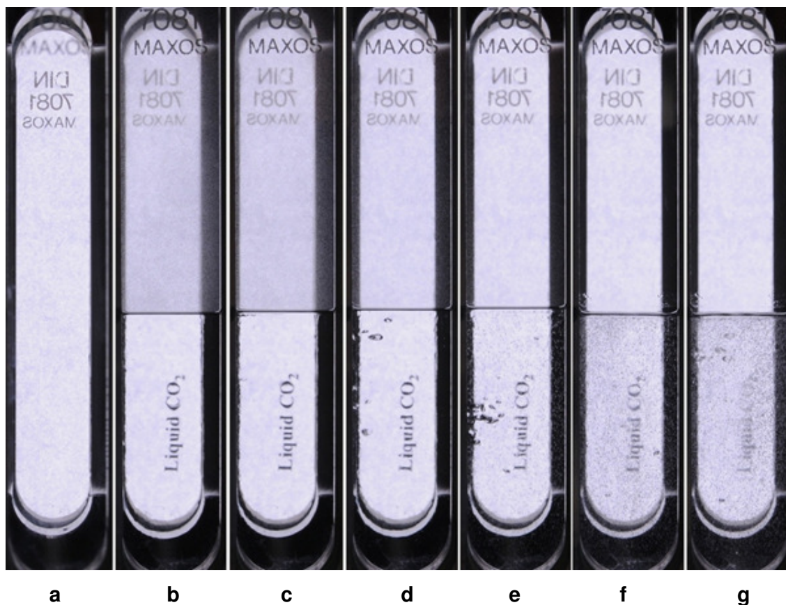
Figure 5.3: Different states of CO 2 in a high pressure cell: a) the cell before filling; b) the cell is filled with CO 2 ; c) bubbling starts at the interface upon decrease of temperature; d) and e) bubble size gets larger with time; f) and g) bubble size decreases while bubble amount increases
