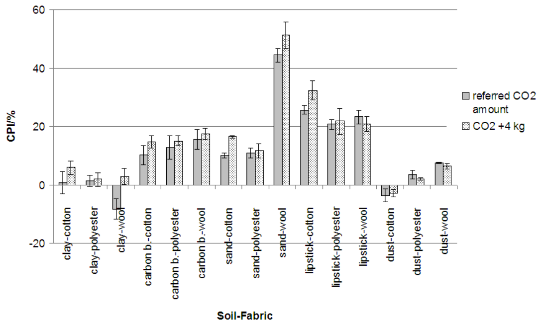
Figure 4.9: Influence of CO 2 amount on CPI
