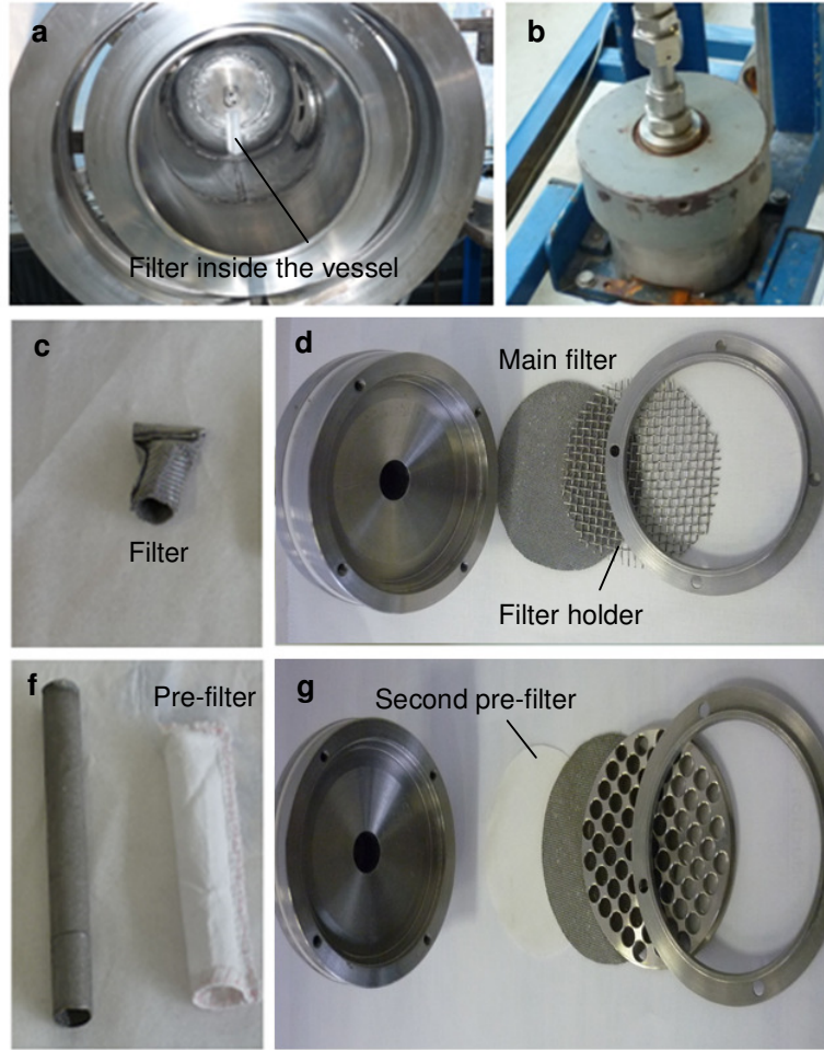
Figure 3.9: The vessel with filter (a); the filter house (b); the existing filtration system: the filter (c) and the main filter (d); the new filtration system: the filter (f) and the main filter (g)
