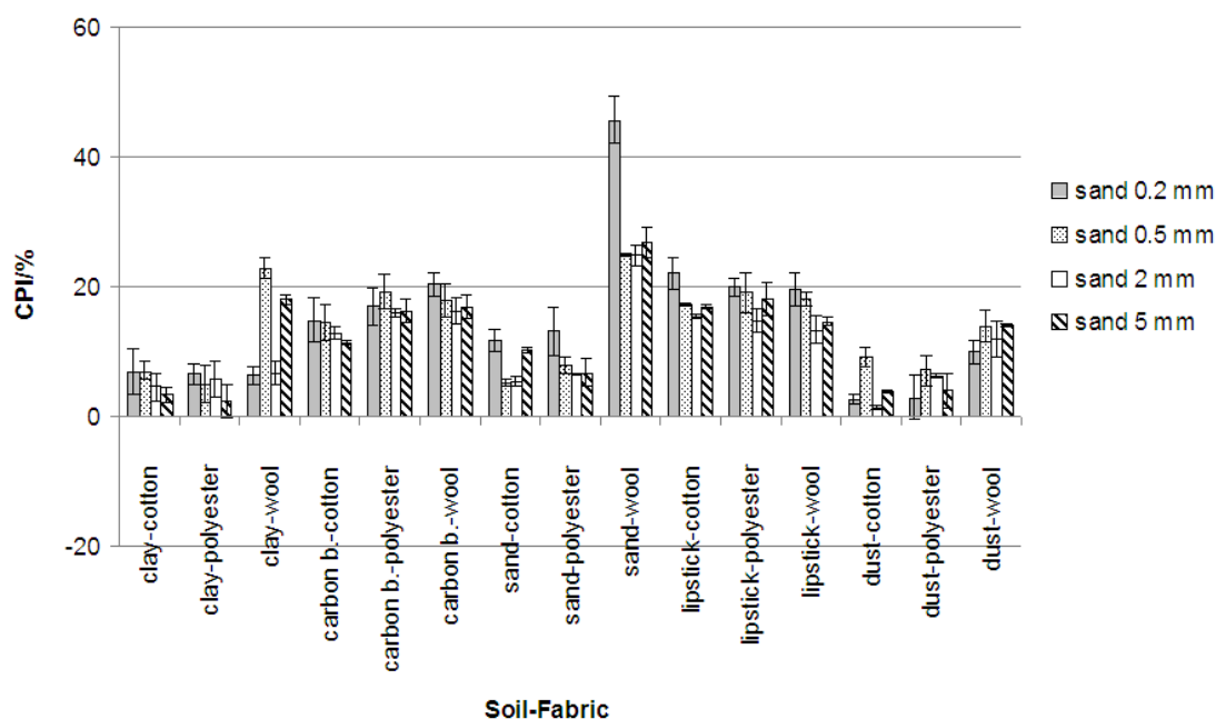
Figure 4.5: Influence of sand diameter on CPI
