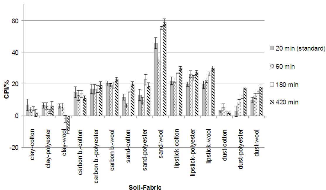
Figure 3.5: Influence of washing time on cleaning result
