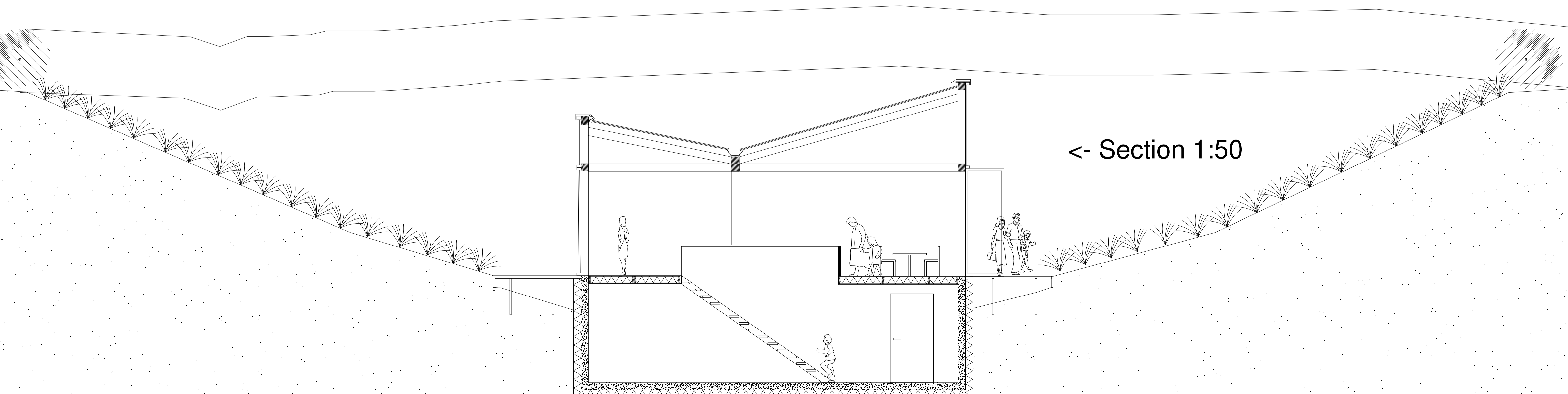
Tunnel Section 1:50
