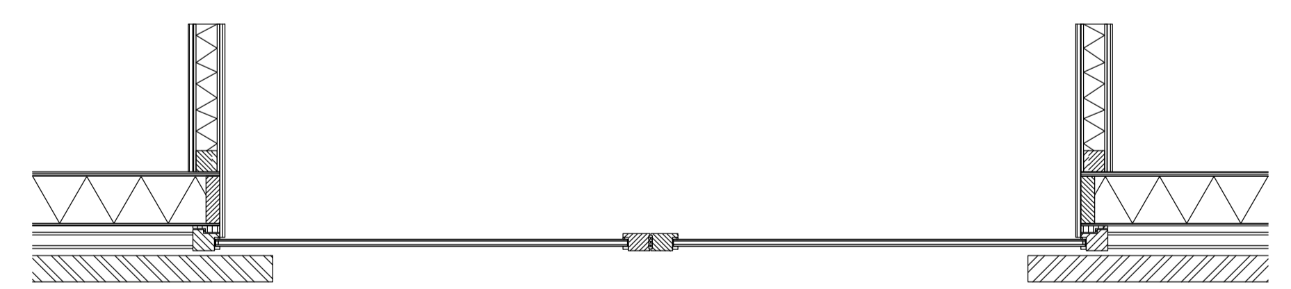
Horizontal Section 1:20
