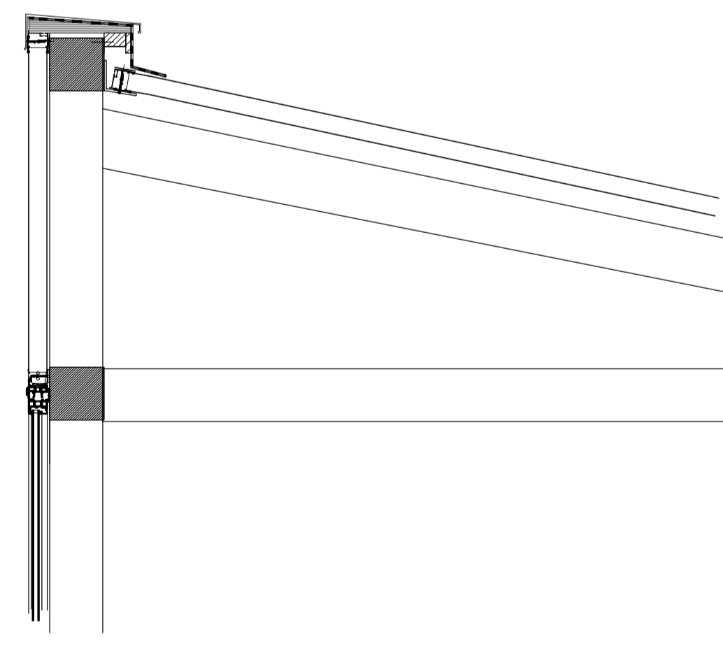
Vertical Section 1:20
