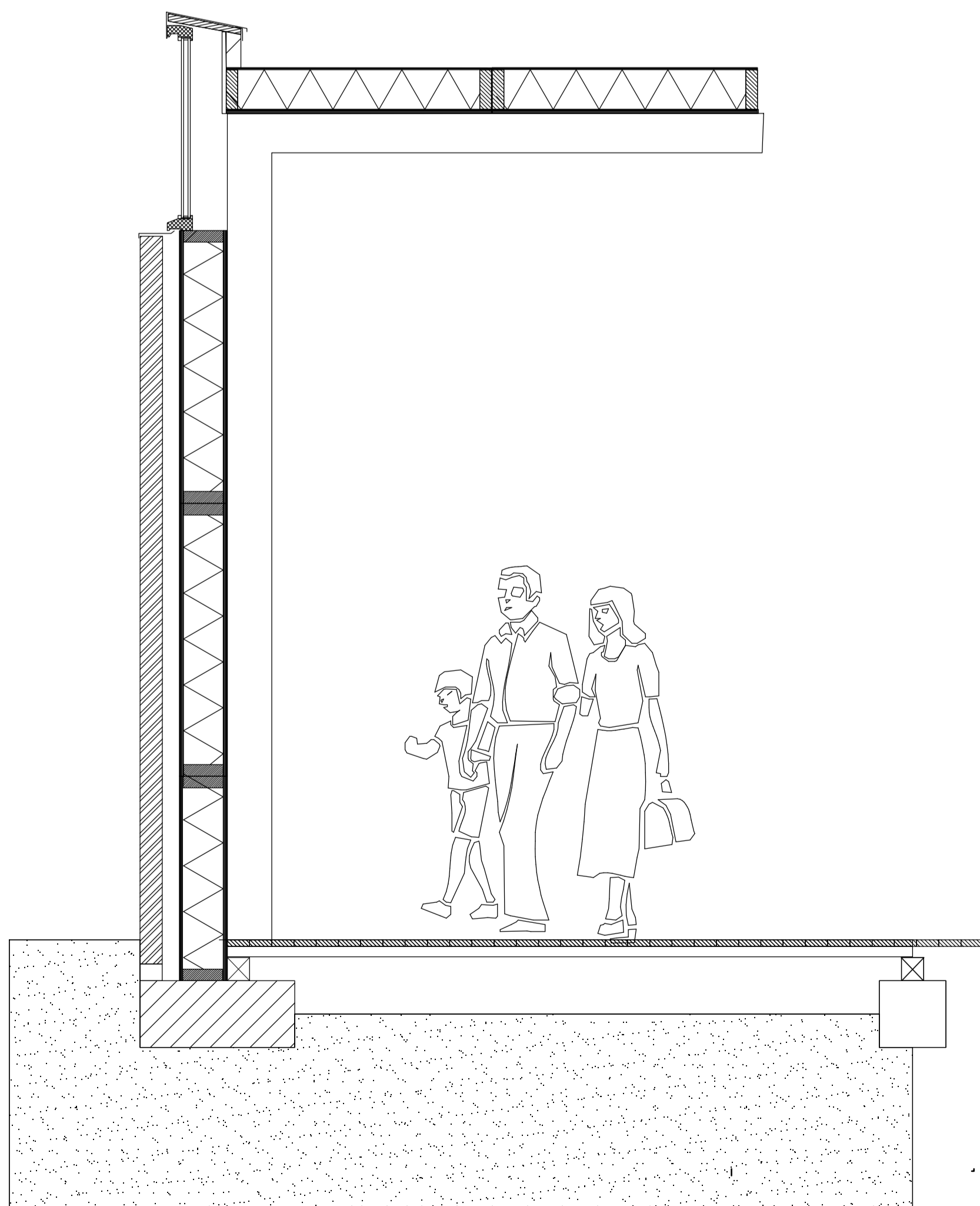
Vertical 1:20
