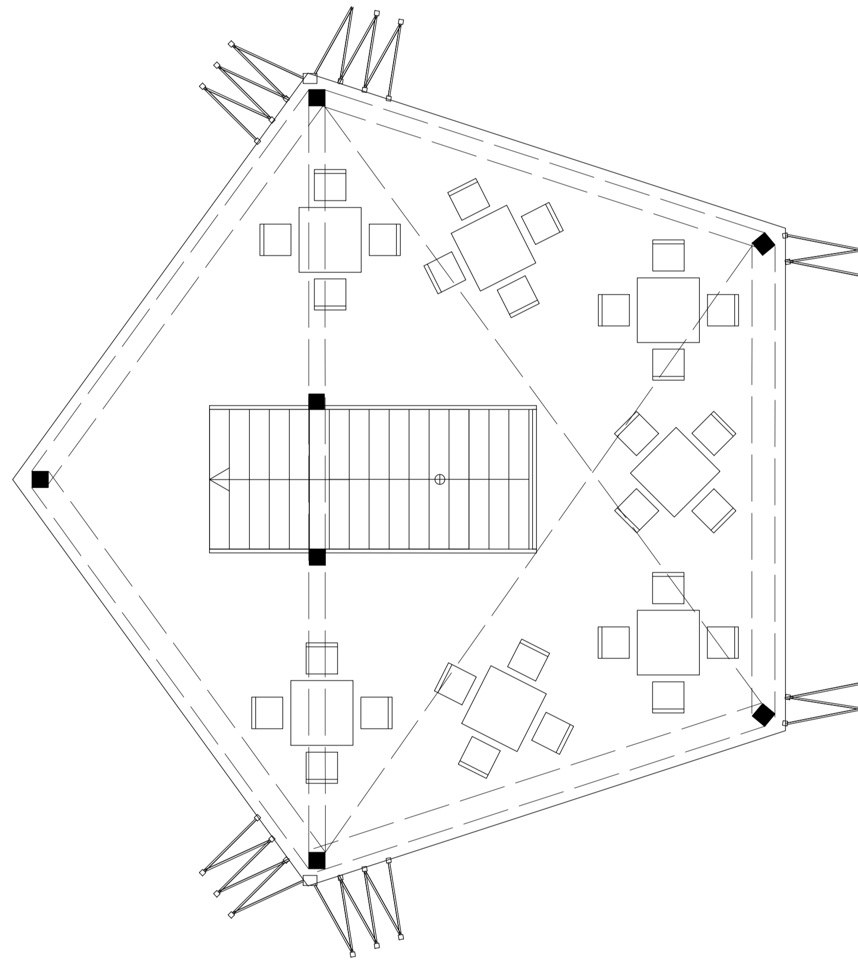
Summer Plan
