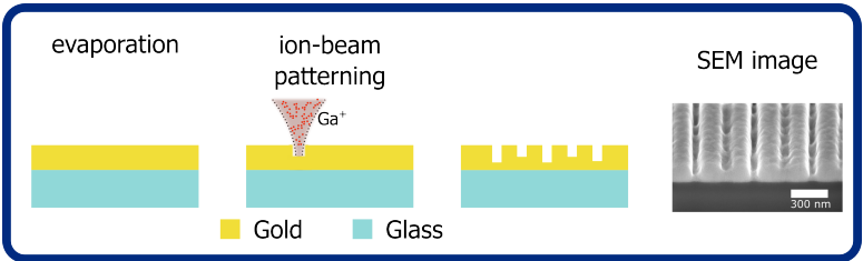
Figure 2.4: Schematic illustrations of the nanofabrication steps using focused ion beam milling to create a nanostructured grating pattern in a gold film. The final illustration shows a scanning electron microscope image of a grating pattern fabricated using focussed ion beam milling.
