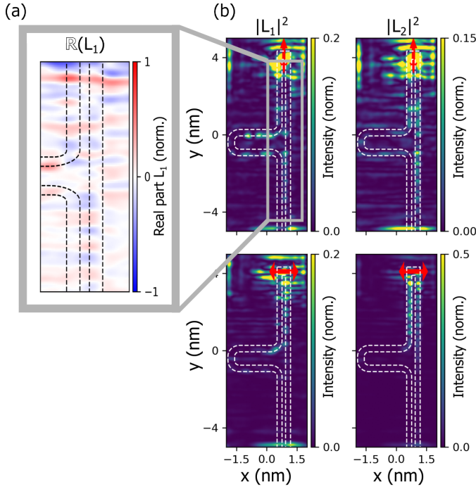
Figure 6.5: (a) False-color plot of the real part of the measured signal L_1 in a plasmonic mode shifter system. (b) Plasmonic field intensities of L_1 (left) and L_2 (right) in the same mode shifter system are indicated by the white dashed line. Light is coupled at the top of the structure to the symmetric (top) and anti-symmetric (bottom) modes.
