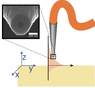
Figure 2.2: Schematic illustration of a collection-type near-field scanning optical microscope probing a plasmonic mode confined to a metallic surface. The inset shows a scanning electron microscope image of a near-field probe.
