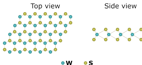
Figure 1.5: Schematic representation of a \text{WS}_2 monolayer from a top and side view.
