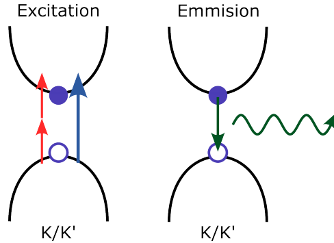
Figure 1.6: Illustration of the photoluminescence process in \text{WS}_2 . Linear (blue arrow) or nonlinear (red arrows) absorption excites excitons at the K and \text{K}' points in the Brillouin zone. Light with the frequency corresponding to the exciton energy is emitted via radiative recombination of the exciton.
