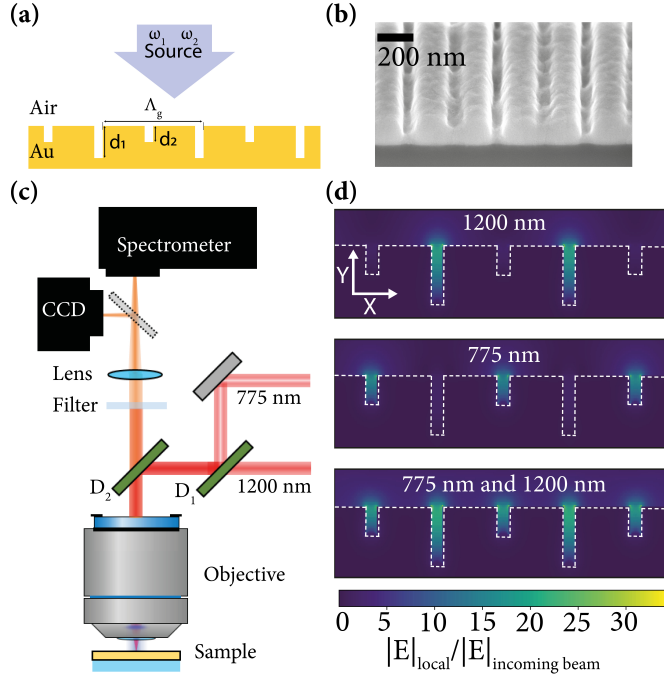
Figure 5.1: (a) Illustration of the double-resonant grating nanostructures gold sample. (b) Scanning electron microscope image of a cross-cut of the double grating nanostructure taken at an angle of 52^\circ . (c) Schematic of the optical setup. (d) Finite-difference time-domain simulations of the electric field, normalized to the electric field of the incoming beams. In the top map the double resonant grating structure is illuminated with a wavelength of 1200 nm and probed at 1200 nm. In the middle map the grating structure is illuminated with a wavelength of 775 nm and probed at 775 nm. In the bottom map we illuminated the grating with both the 775 nm and 1200 nm beams, the local field is evaluated separately at both wavelengths afterwards these two images are merged together.
