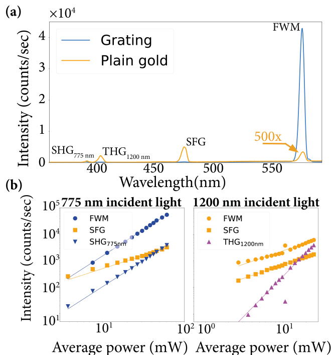
Figure 5.3: (a) Spectra of the generated signal on a gold surface (orange) and the double nanostructure grating etched in gold (blue). SHG 775 nm , THG 1200 nm , SFG and FWM are observed on plain gold and the nanostructure. (b) Double logarithmic plot of the intensity of the nonlinear signals in gold as a function of the power of the incoming beams. The power functions of the nonlinear effects appear as straight lines on the double logarithmic scale where the slope corresponds to the power order of the nonlinear effect. Linear (orange), quadratic (blue) and cubic (pink) monomial functions are fitted through the data points.
