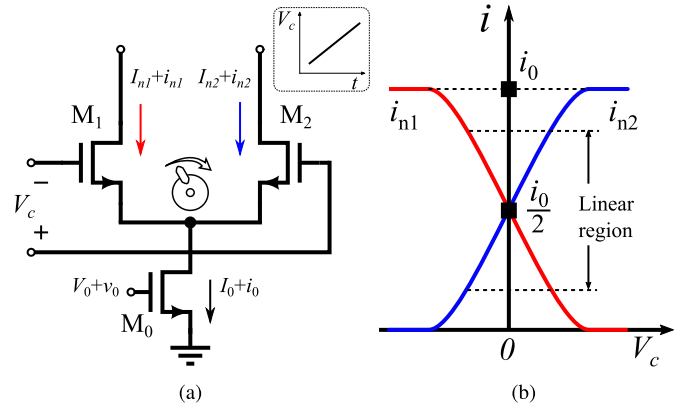
Fig. 4. (a) NMOS current-steering pair with inset showing the control voltage as a function of time. (b) AC currents of NMOS pair as a function of control voltage V_c .
