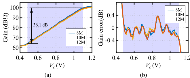
Fig. 11. (a) Measured AFE gain at three frequencies as a function of V_c . (b) Calculated linear-in-dB gain errors.
