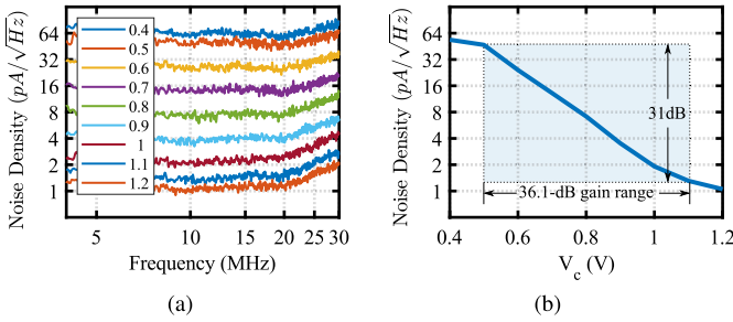
Fig. 14. (a) Measured input-referred noise spectra, (b) Measured in-band noise density as a function of TGC control voltage V_c .
