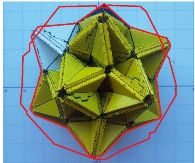
Figure 8. Comparison of the expanded and contracted state of the physical model. The contracted state is shown, with the contours of both the contracted and the expanded state drawn in red.
