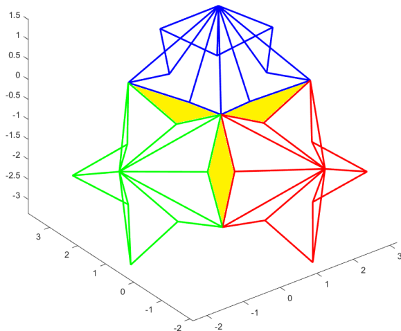
Figure 3. The origami-inspired structure consists of rigid triangular faces, which are connected by folds into pentagonal units (shown with red, blue and green outlines). These units are subsequently coupled by spherical joints, allowing for open spaces (shown in yellow) when the structure is deformed.
