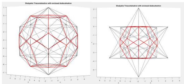
Figure 6. The volume change of the mechanism is determined based on the inscribed dodecahedron, defined by the connection points of the pentagonal units. This dodecahedron is shown here in red.
