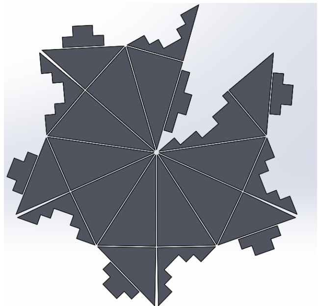
Figure 4. A top view of the pentagonal unit design. These structures were 3D printed in the shown flat state. Netting was used to create fold lines between the grey rigid plates and twelve of these units were assembled into a Dysdiakis Triacontahedron by matching and gluing the notched parts.
