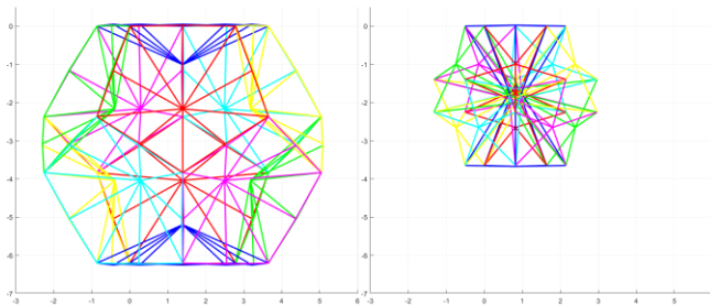
Figure 9. An alternative design, where the pentagonal units are inverted to point into the enclosed volume, for improved scaling of the circumscribed volume. Shown are both the expanded (left) and the contracted state (right).
