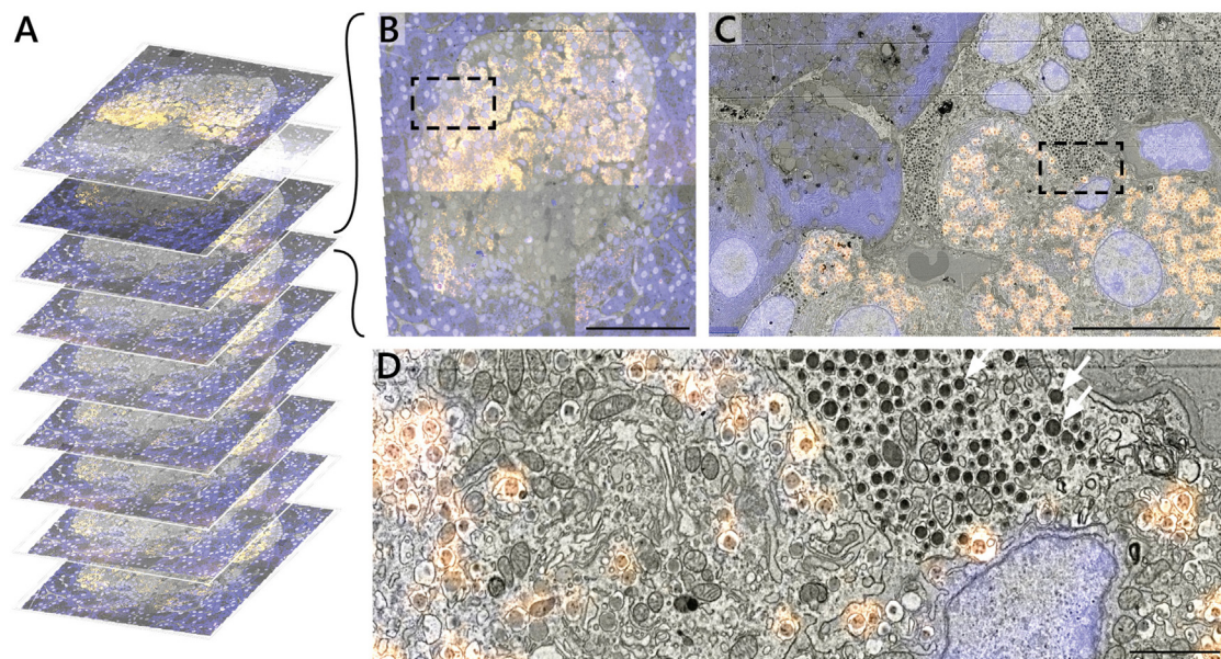
FIGURE 5 | Correlative reconstruction of nine sections of pancreas. (A) 2D and 3D alignment routines are combined to yield a CLEM stack of nine serial sections of rat pancreas tissue. (B–D) CLEM imaging of the islet of Langerhans at varying spatial resolution. Hoechst (blue) and AF594 (orange) fluorescence signals are superimposed onto the EM ultrastructure. The AF594 signal, in particular, facilitates recognition of insulin granules from e.g. non-fluorescent glucagon granules (white arrows, D). Scale bars: (B) 50µm; (C) 5µm; (D) 1 µm. Raw data at full resolution is available via Nanotomy.
