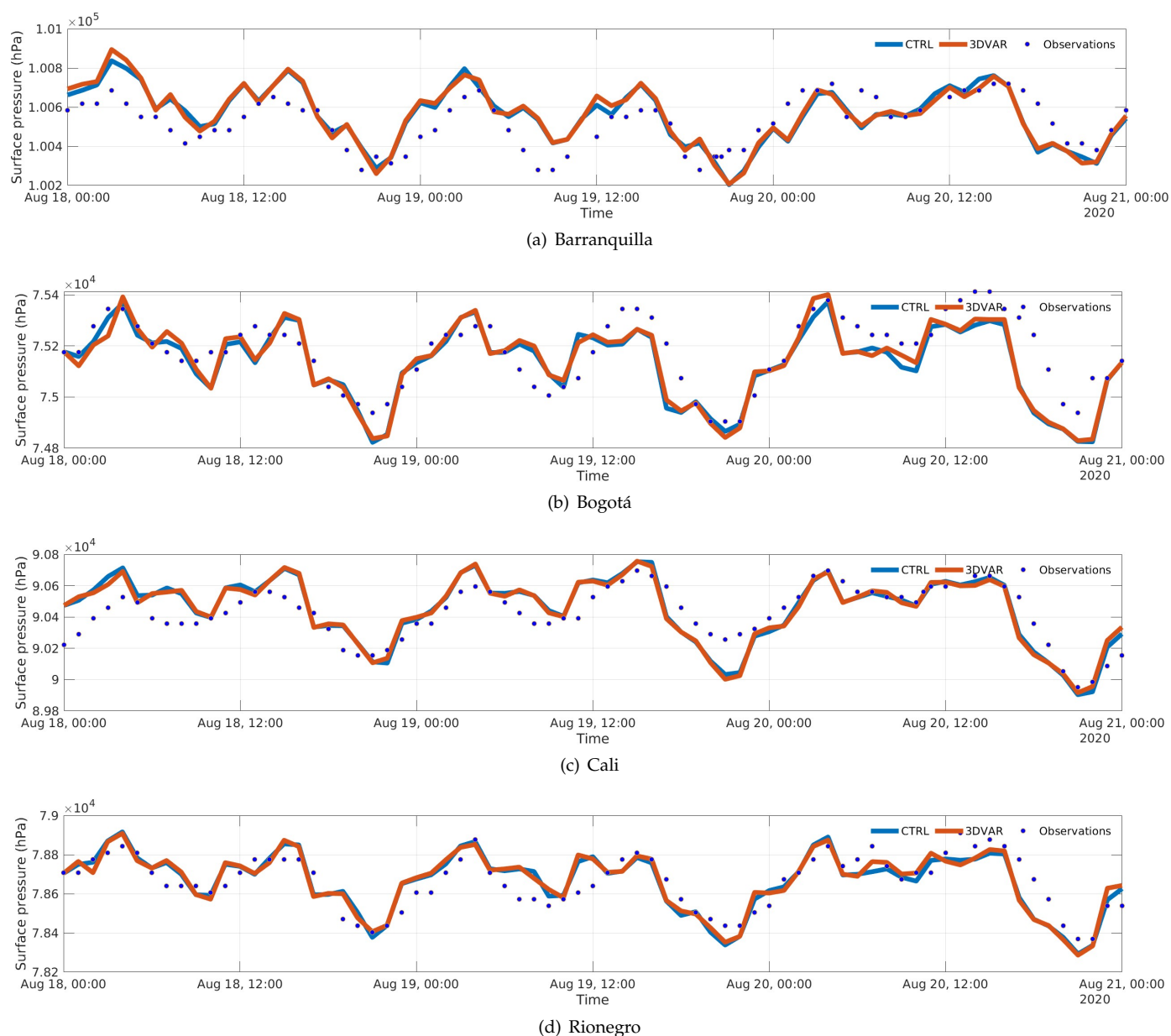
Figure 5. Representation of the surface pressure for the METAR data, 3DVAR, and CTRL in W1 for (a) Barranquilla, (b) Bogotá, (c) Cali, and (d) Rionegro for the forecast window W1.
