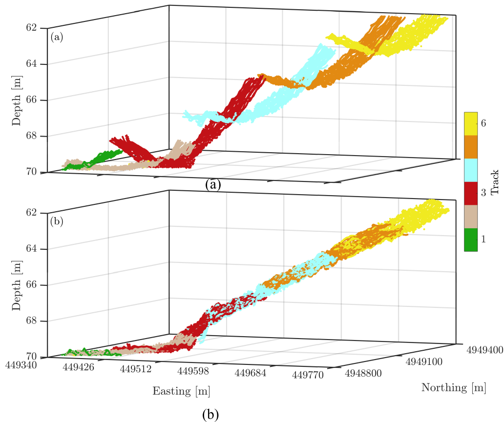
FIGURE 16. Depths within the area consists of 20 pings indicated as 1 in Fig. 15 based on the (a) measured SSPs and (b) result of DE based SSP inversion. Varying colors indicate different sailed tracks.
