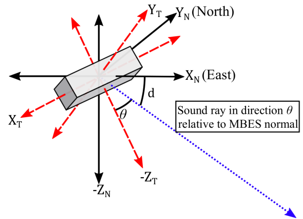
FIGURE 1. MBES measurement configuration schematic. X_T , Y_T and Z_T denote the transducer frame. X_N , Y_N , Z_N indicate the navigation frame. \theta and d are the beam angles of the sound ray relative to the MBES normal and navigation horizontal plane respectively.
