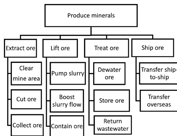
FIGURE 2 Functional architecture of the material flow in offshore operations during exploitation.
