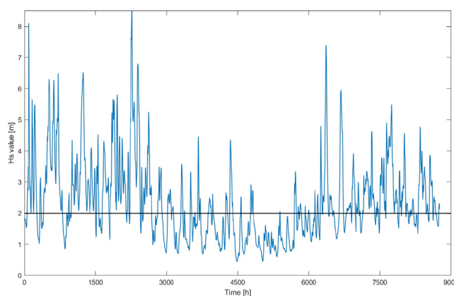
FIGURE 5 Hindcast time series for significant wave height ( H_s ) in the Norwegian Sea during the year 2021. A 2 m maximum threshold is included for illustration purposes. Generated using Copernicus Climate Data, 27 accessed 2022-08-19.
