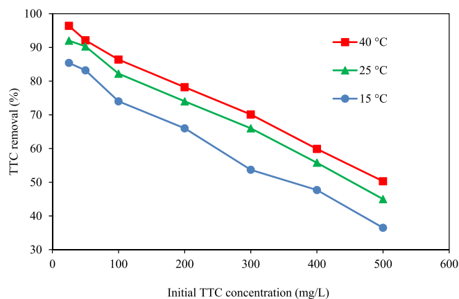
Fig. 6. Effect of solution temperature on TTC removal at different initial TTC concentration at pyrite/H 2 O 2 process (Reaction conditions: pH: 4.1, H 2 O 2 concentration: 5 mmol/L, pyrite dosage: 1 g/L, reaction time: 120 min).
