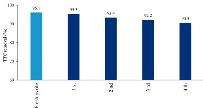
Fig. 8. The reusability and durability of pyrite for TTC degradation (pH: 4.1, \text{H}_2\text{O}_2 concentration: 5 mmol/L, pyrite dosage: 1 g/L, reaction time: 120 min).
