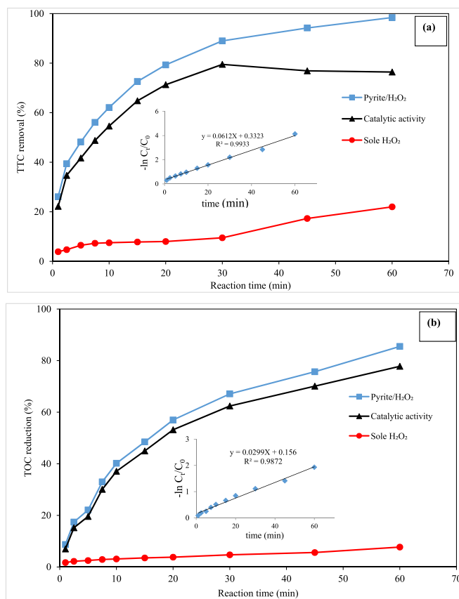
Fig. 7. Catalytic activity of pyrite for (a) TTC degradation and (b) TOC reduction in the pyrite/ \text{H}_2\text{O}_2 process as a function of contact time (pH: 4.1, \text{H}_2\text{O}_2 concentration: 5 mmol/L, pyrite dosage: 1 g/L, initial TTC concentration: 50 mg/L).
