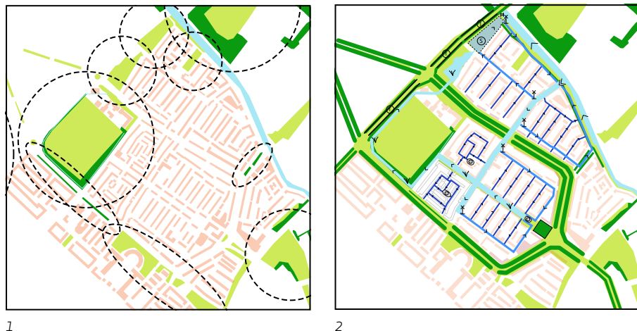
FIGURE 8.16 1. Green in Ondiep with a circle of 200 meters from the green; 2. Design for green zones and an integral water system.
